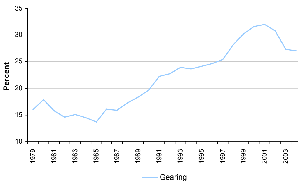
Figure 5 – Gearing ratio: 1979-2004
