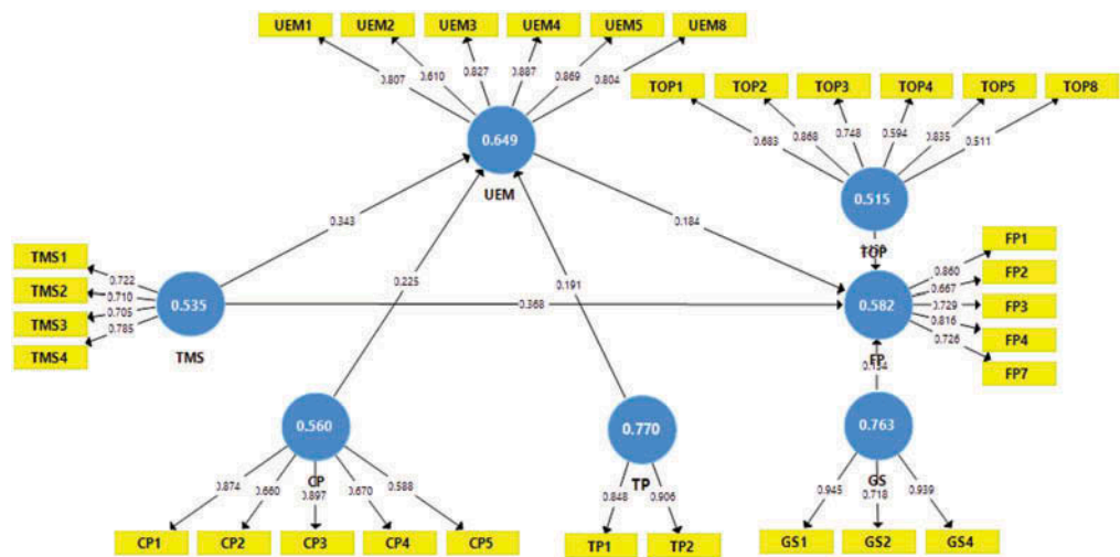
Figure 2. Measurement model —factor loadings and coefficients values.
