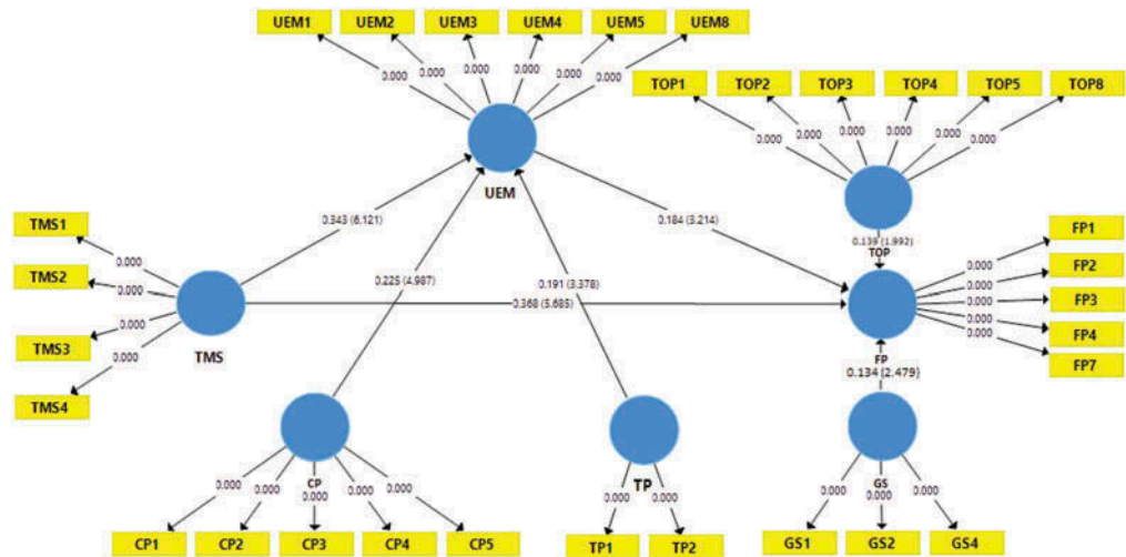
Figure 3. Measurement model —significance values and T-statistics.
