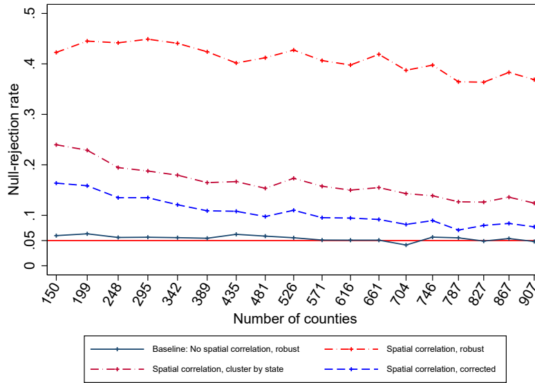
(a) OLS
