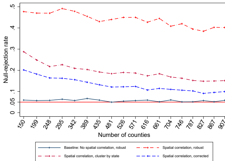
(b) 2SLS
