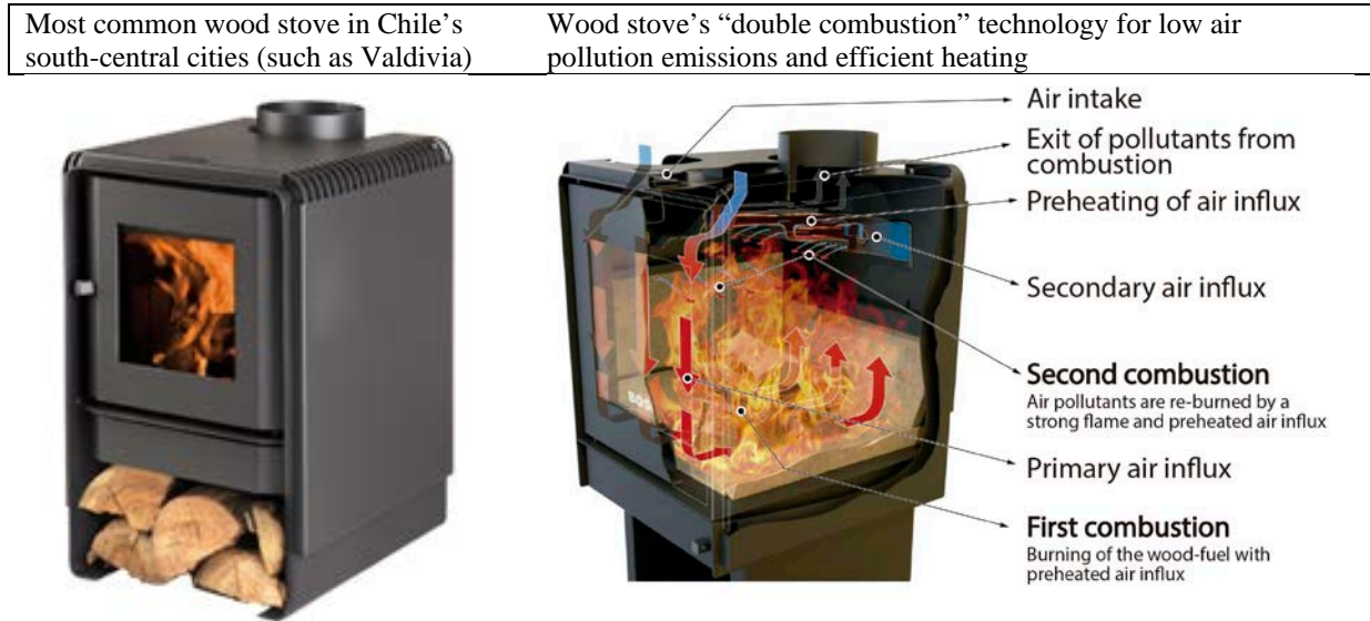
Figure 2. Wood Stoves' Combustion Technology and Outdoor Pollution Emissions
