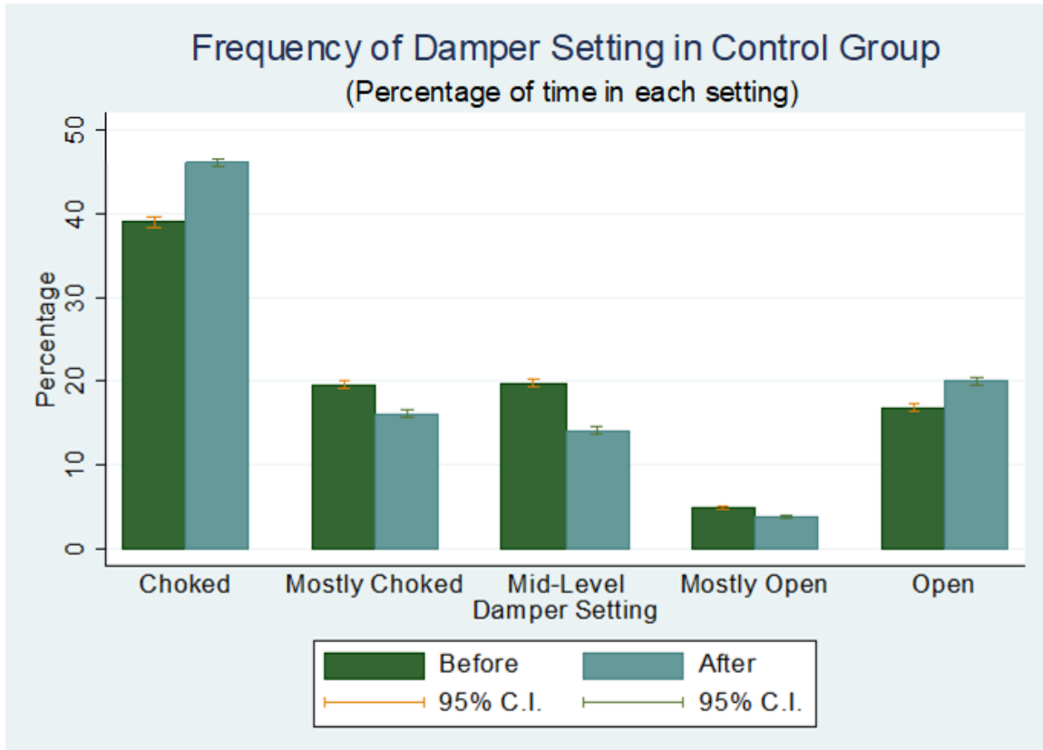
Figure 8. Frequency of Damper Setting for Control Group, Percentage of Time the Wood Stove Is On
