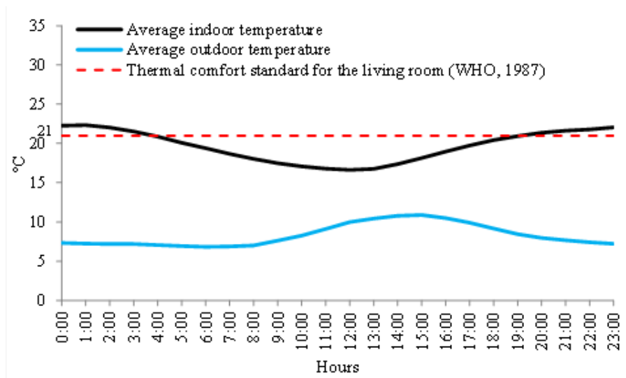
Figure 6. Indoor and Outdoor Temperature Profile for Participating Households in Valdivia, Chile: Average for August and September 2017
