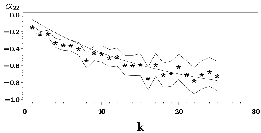
Figure B18: \alpha 's of the model with 6 zero restrictions.
