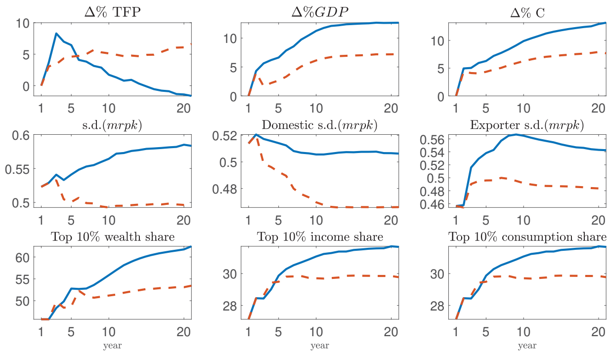
Figure 5: Transition dynamics after trade liberalization with closed (dashed line) or with open capital markets
