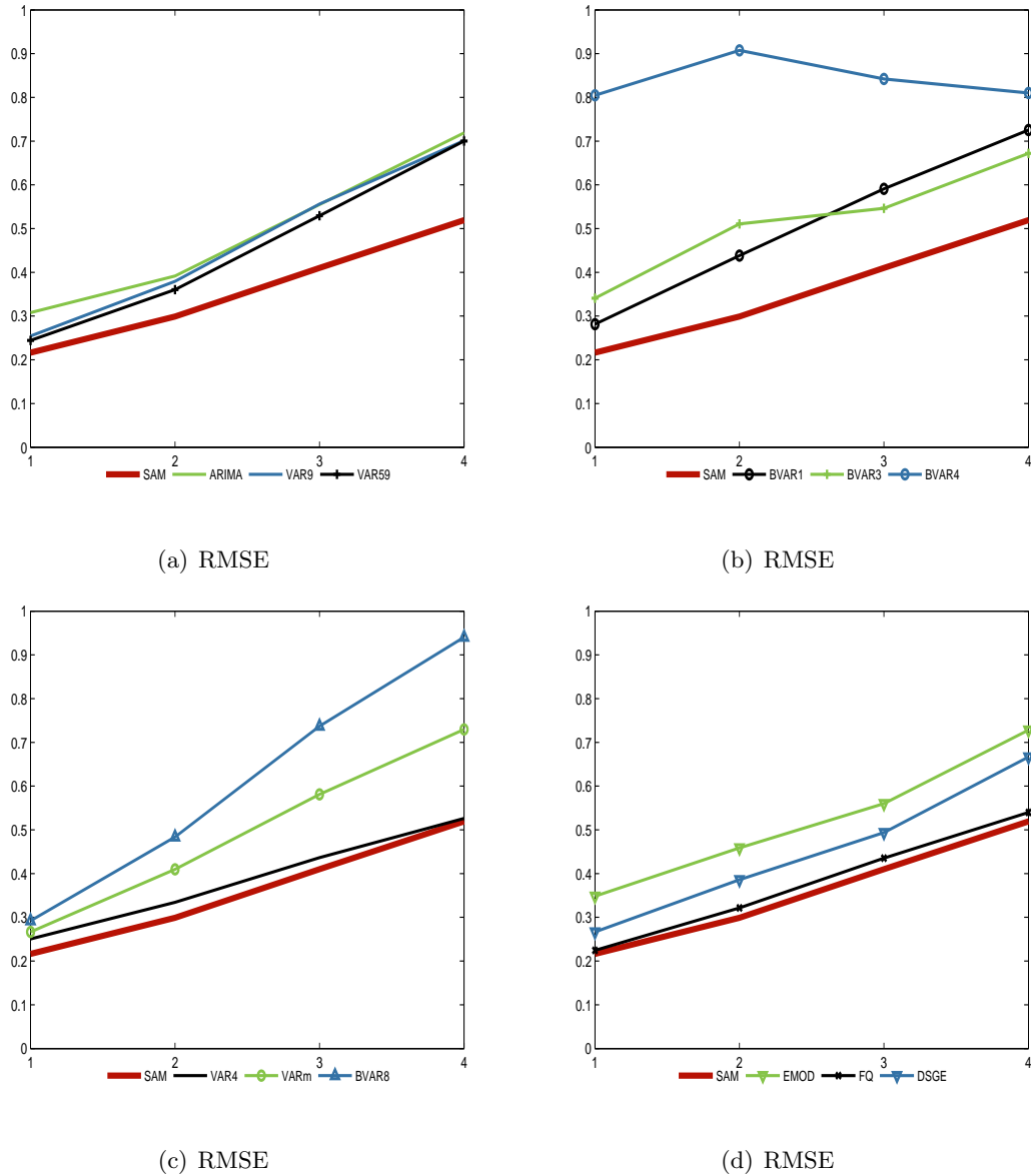
Figure 2: RMSE for inflation
