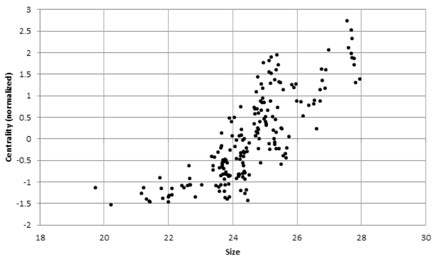
Figure 3: Cross plot of centrality and size; the correlation is 0.80. Asset values in logs measured at end of each quarter over the period 9 October 2006 to 6 April 2009.
