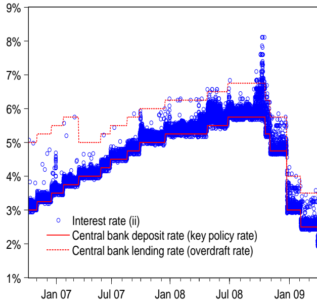
Figure 2: Interest rates on identified loans (ii) and the central bank’s deposit and lending rates. The spread between the latter interest rates has been one percentage point since 16 March 2007. Daily observations over the period 9 October 2006 to 6 April 2009. Interest rates in % per annum.
