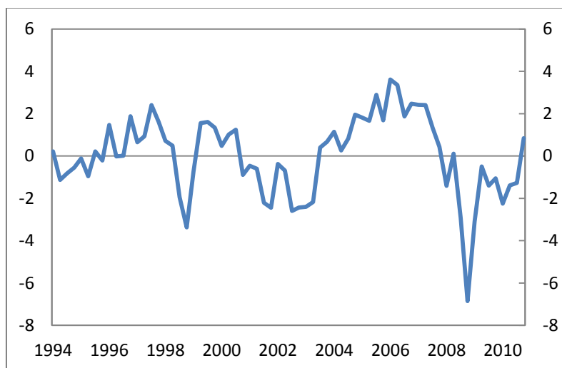
Figure 5.4: First principal component (PC1Q), quarterly series. 1994Q1-2010Q4.
