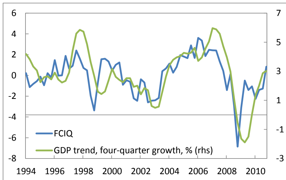
Figure 6.2: Quarterly FCI and four-quarter growth in trend GDP (%). 1994Q1-2010Q4.
