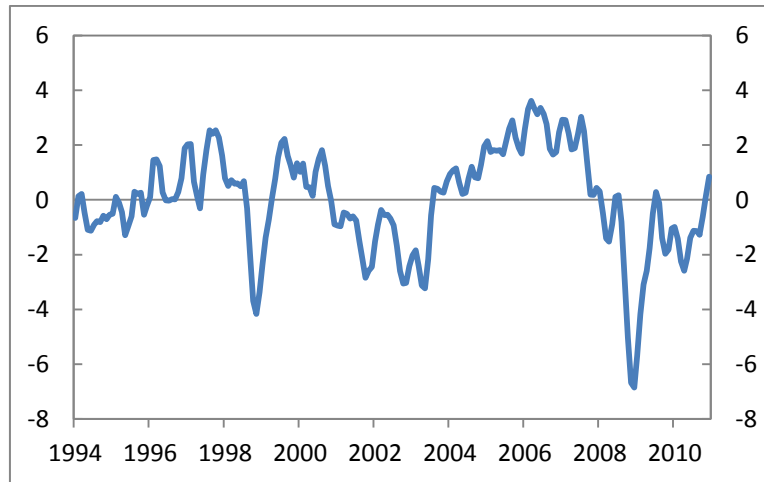
Figure 5.1: First principal component, monthly series. 1994M1-2010M12
