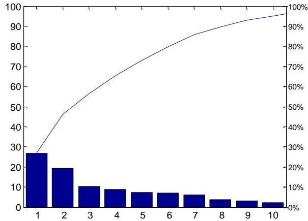
Figure 5.2.: Per cent of total variance explained by each of the first 10 principal components and cumulative variance accounted for by the same 10 principal components.
