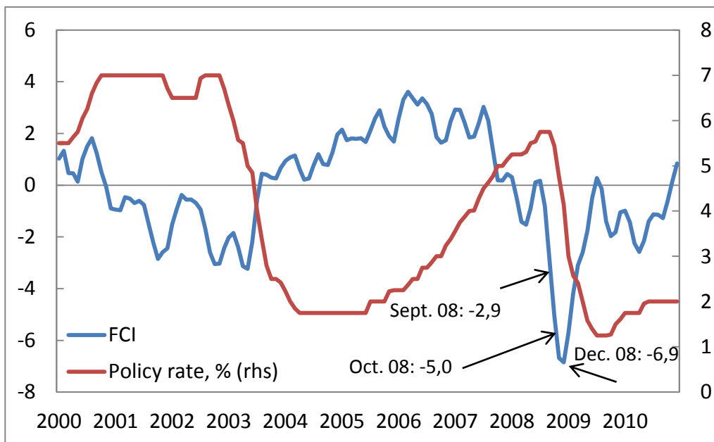
Figure 6.5: FCI and the key policy rate (%), monthly series. 2000M1-2010M12.
