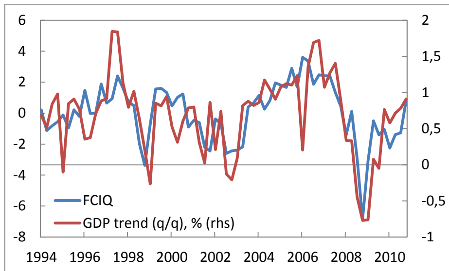
Figure 6.1: Quarterly FCI and quarterly growth in trend GDP (%). 1994Q1-2010Q4.
