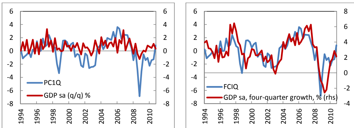
Figure 5.5a and b: First quarterly principal component (PCQ1) and a) quarterly GDP growth, sa (%) b) four-quarter GDP growth, sa (%).1994Q1-2010Q4
