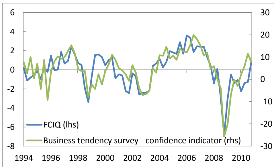
Figure 6.3: FCI and the Business tendency survey confidence indicator, unadjusted. Quarterly series. 1994Q1-2010Q4.
