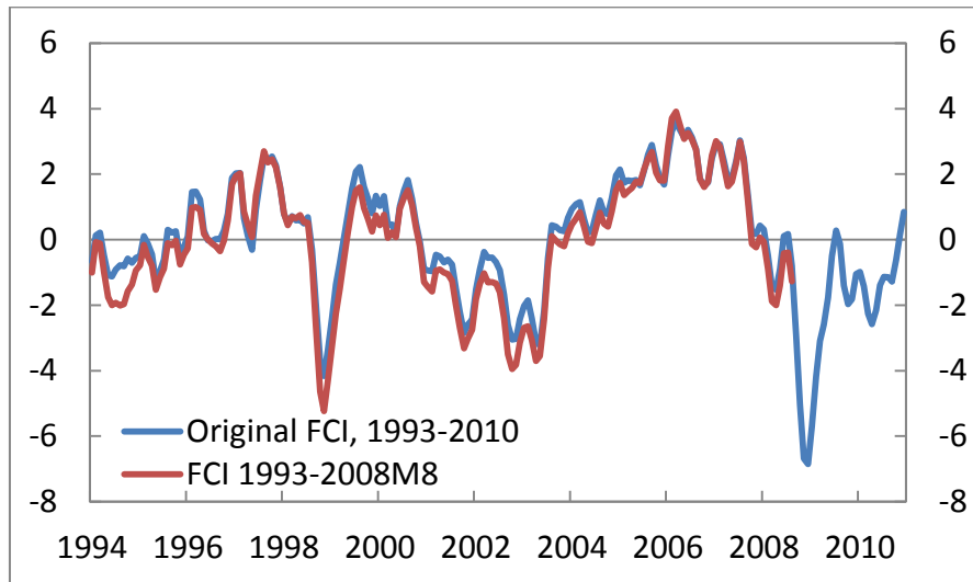
Figure 6.6: Original FCI and FCI based on data from 1993M1-2008M8, monthly series. 1994M1-2010M12. (The periods indicated in the legend refer to the data periods covered).
