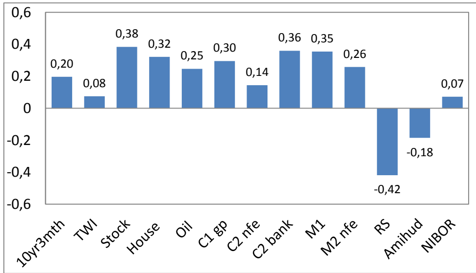
Figure 5.3: Factor loadings, first principal component.
