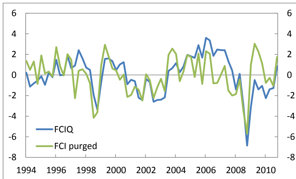
Figure 6.4: Comparison of FCIs, purged and unpurged quarterly series. 1994Q1-2010Q4.
