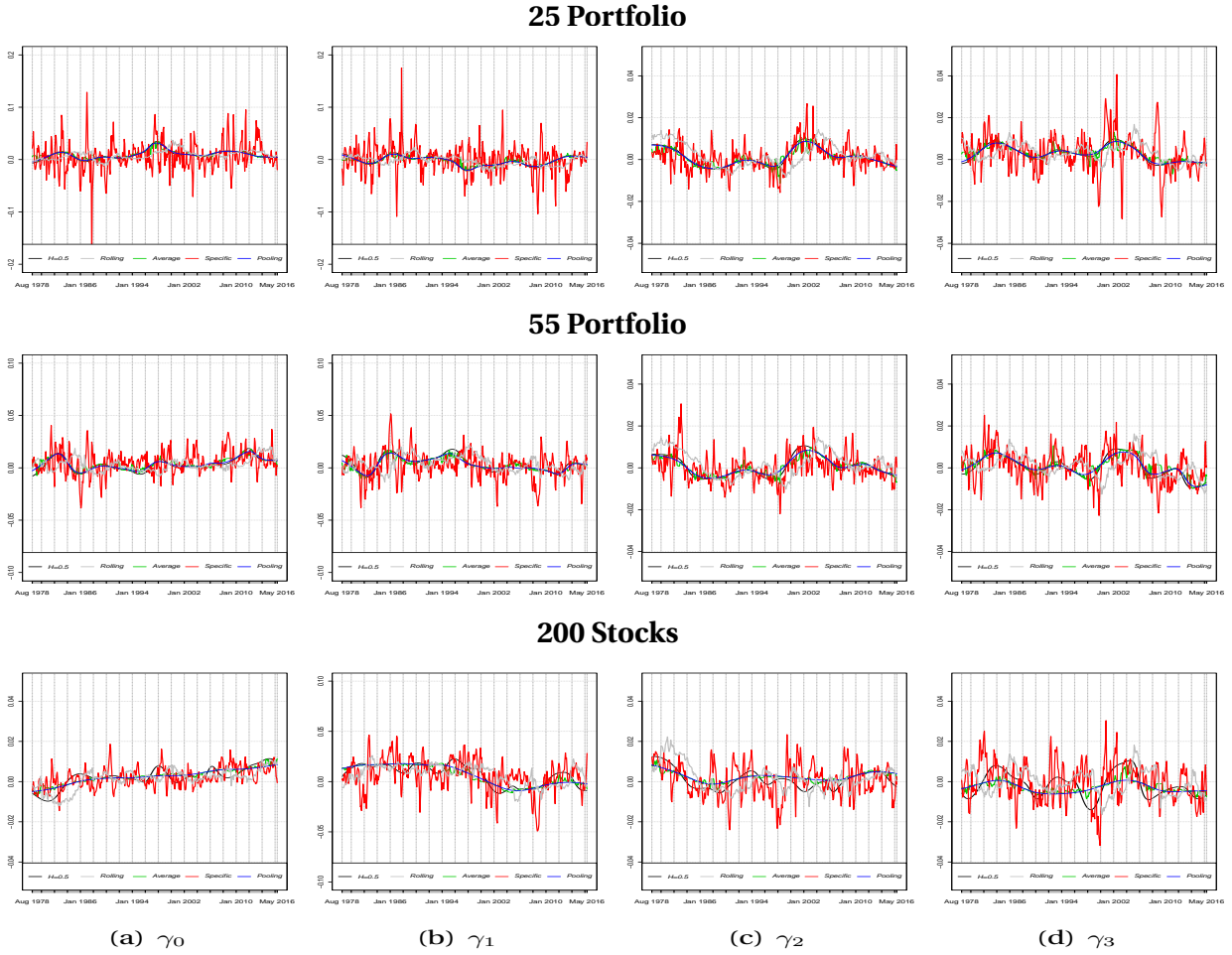
Figure 3: Dynamic comparison of risk premia estimates for different approaches
