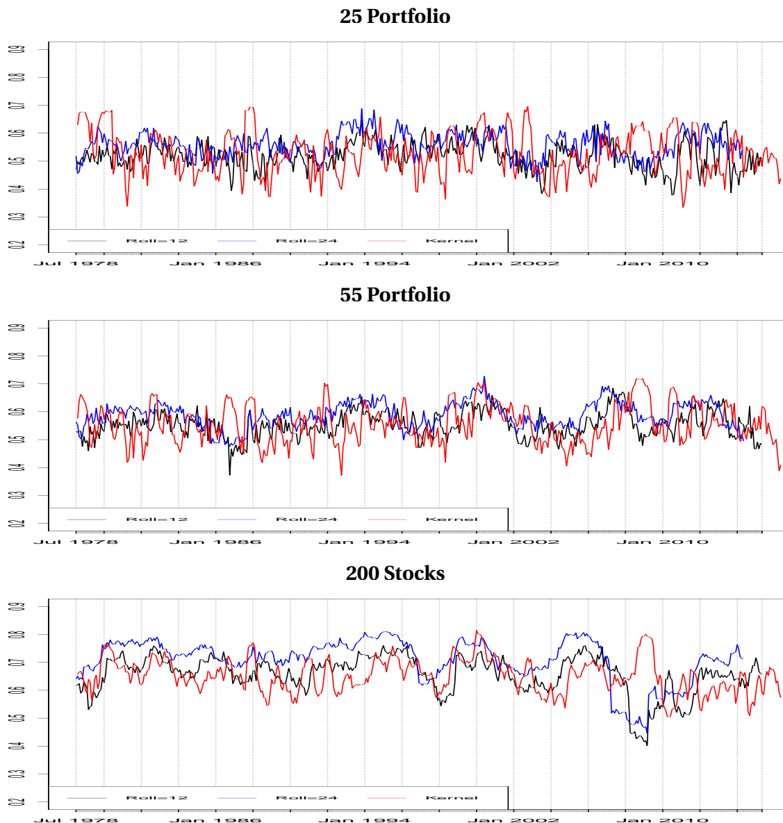
Figure 1: Time Varying optimal bandwidth parameter
