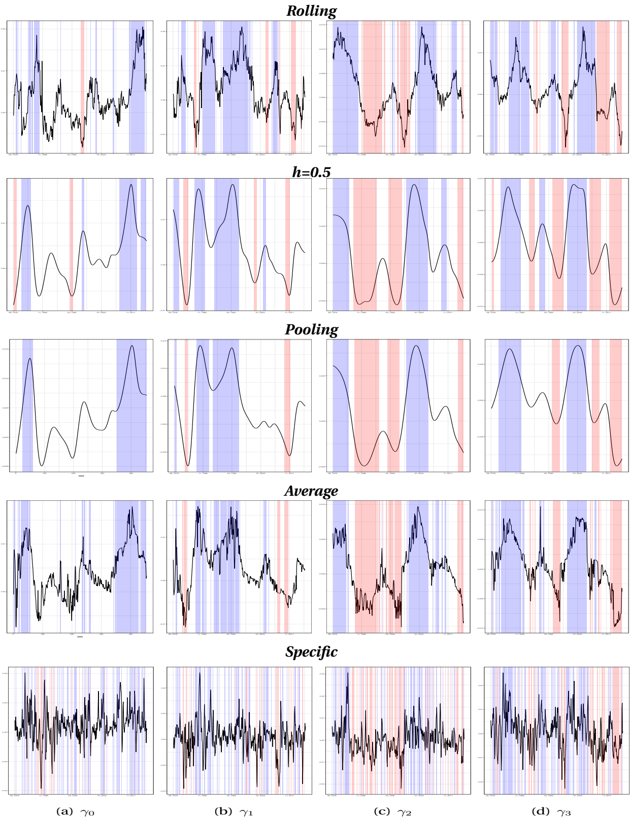
Figure 5: Comparison of gammas significance of different approaches - 55 Portfolios
