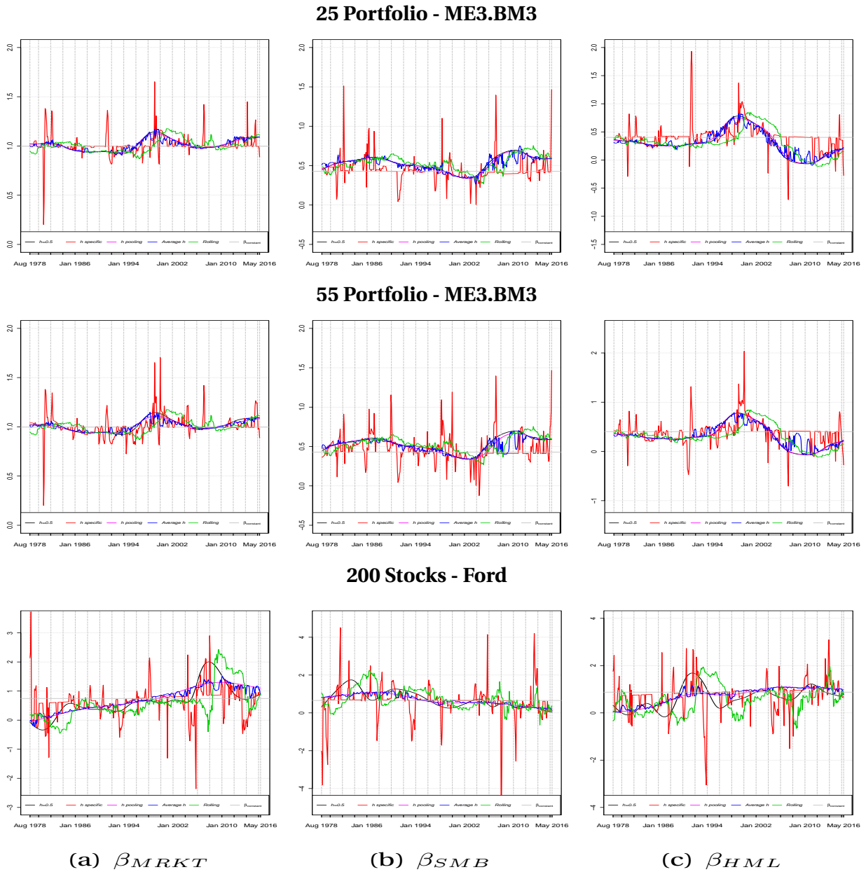
Figure 2: A dynamic comparison of the factor loading estimates
