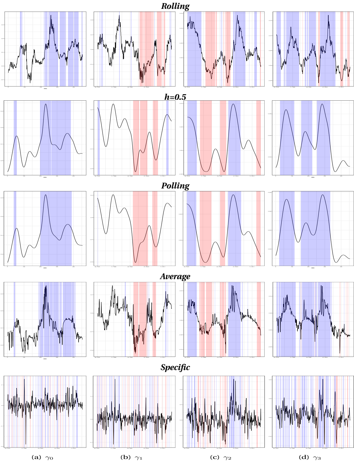
Figure 4: Comparison of gammas significance of different approaches - 25 Portfolios
