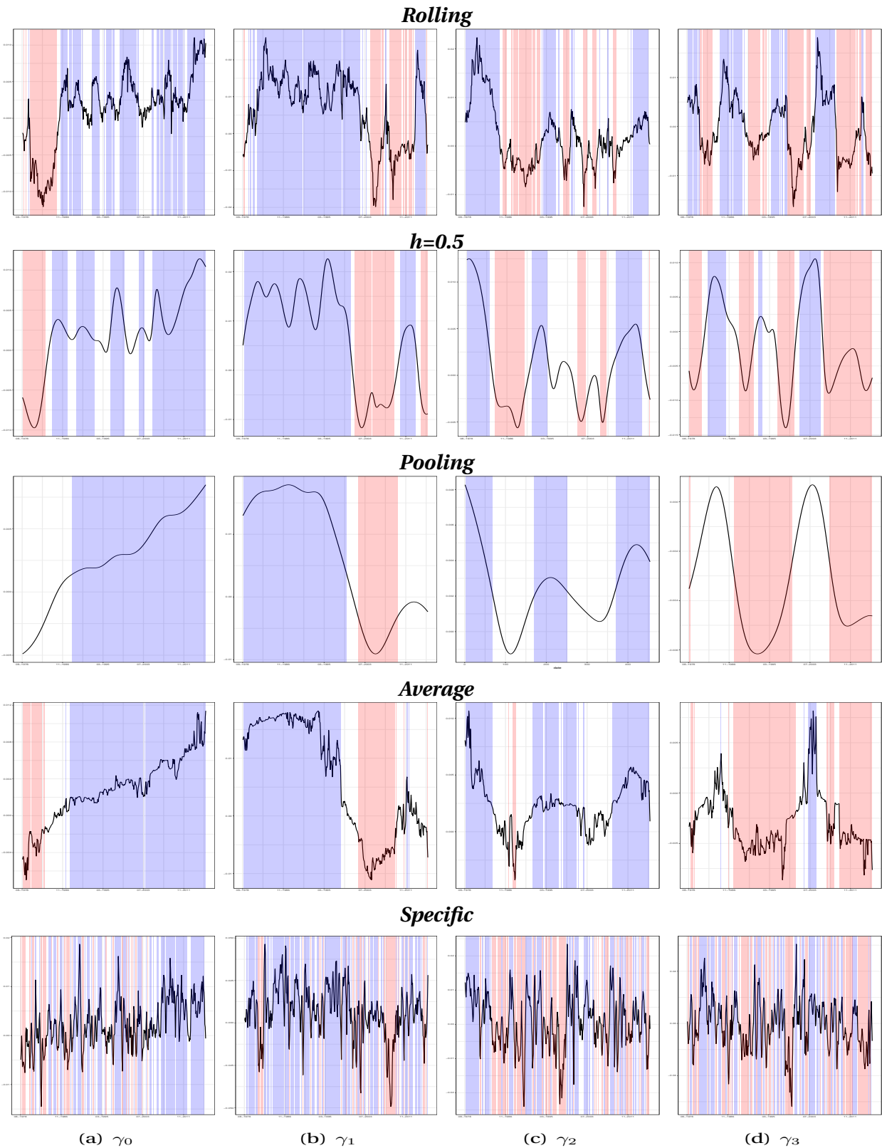
Figure 6: Comparison of gammas significance of different approaches - Individual stocks
