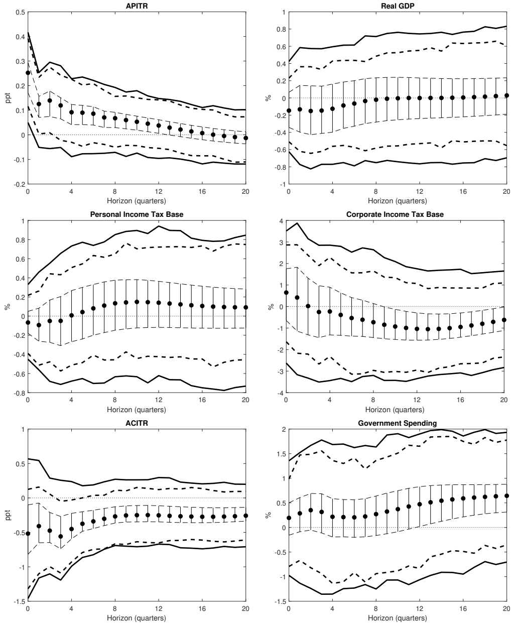
Figure 2: Impulse Responses to \varepsilon_{APITR,t} Under Set-Identifying Restrictions (Single and Multiple Priors)
