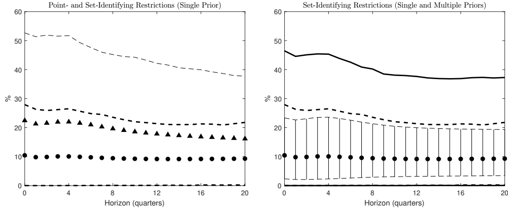
Figure 5: Contribution of \varepsilon_{APITR,t} to Forecast Error Variance of Real GDP
