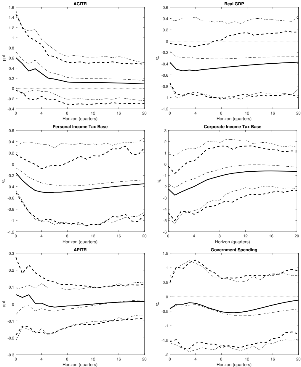
Figure 3: Impulse Responses to \varepsilon_{ACITR,t} Under Different Identifying Restrictions (Single Prior)
