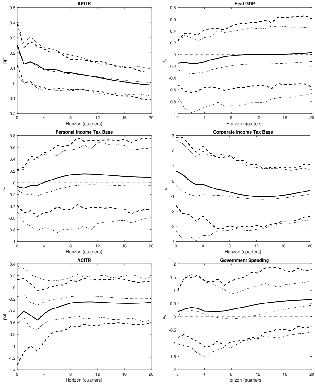
Figure 1: Impulse Responses to \varepsilon_{APITR,t} Under Different Identifying Restrictions (Single Prior)
