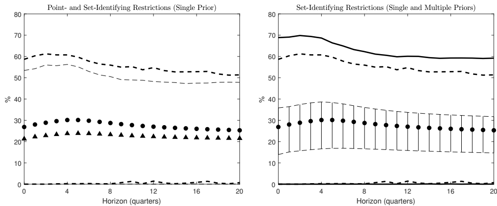
Figure 6: Contribution of \varepsilon_{ACITR,t} to Forecast Error Variance of Real GDP
