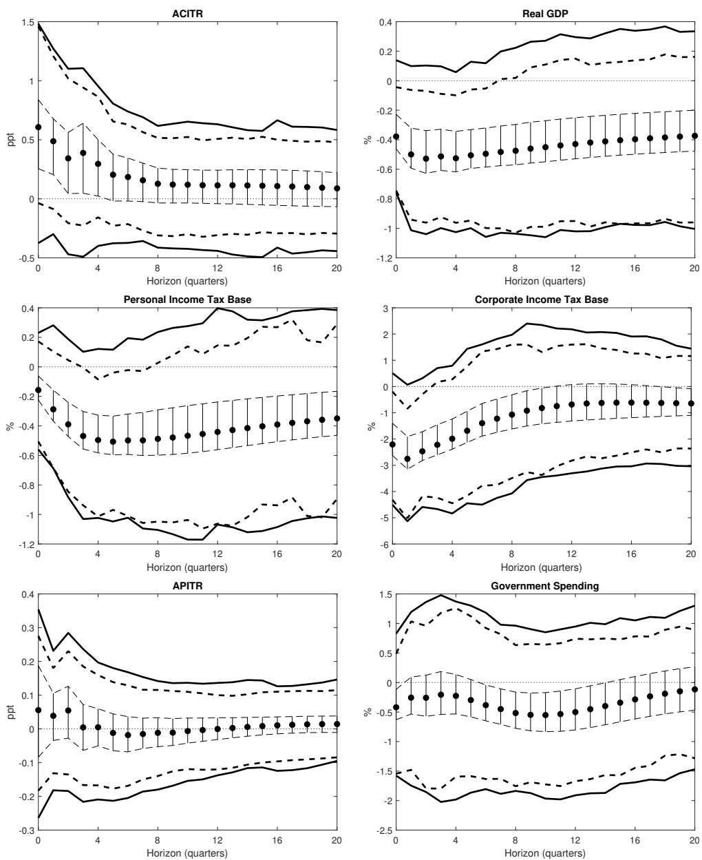
Figure 4: Impulse Responses to \varepsilon_{ACITR,t} Under Set-Identifying Restrictions (Single and Multiple Priors)
