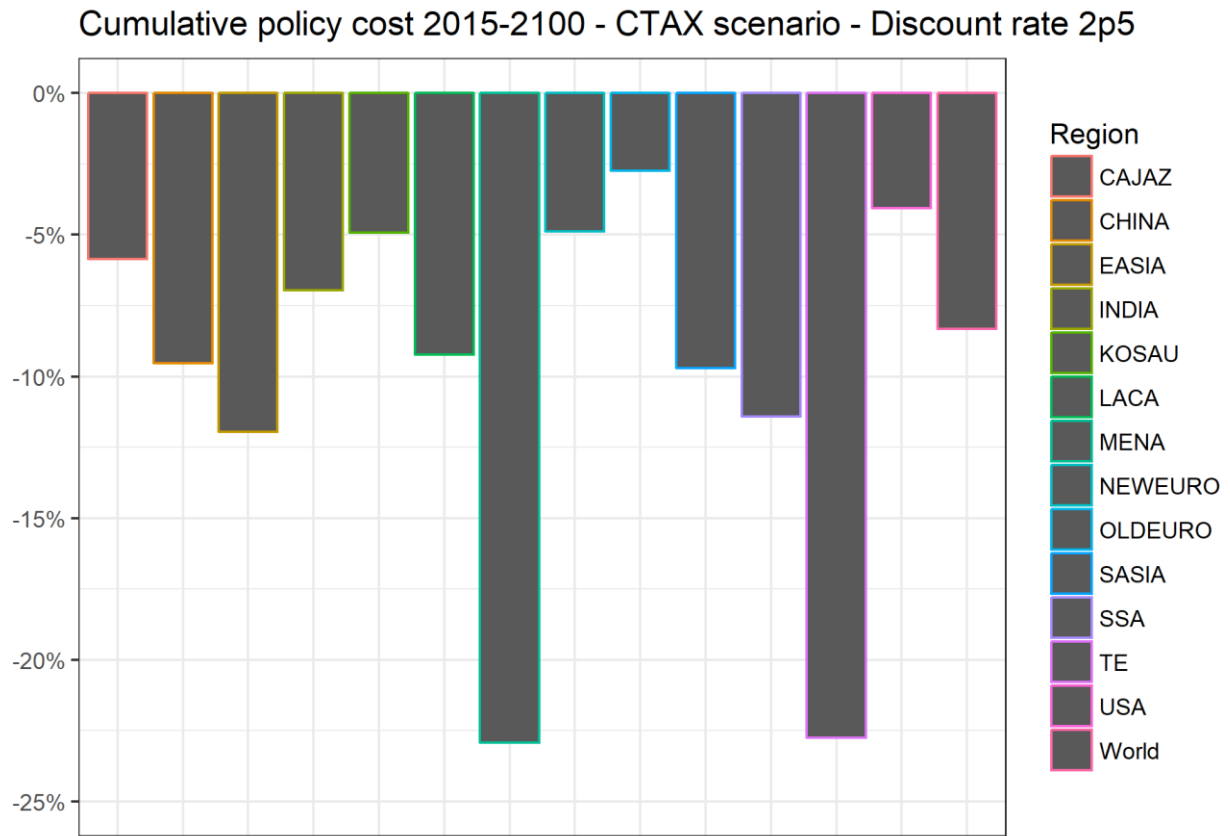
Figure 16 – Regional policy costs in the CTAX scenario.
