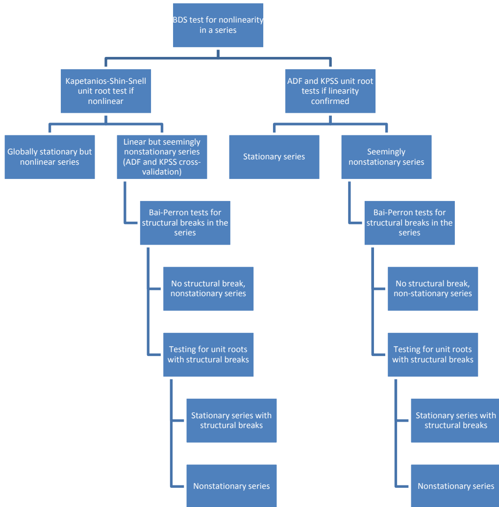
Figure 1 Unit root testing scheme for VAR models.
