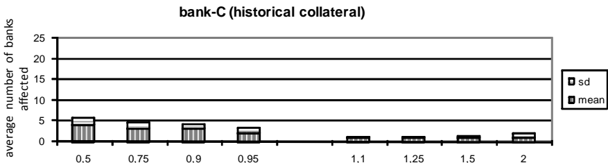
Figure 5.9 Average number of bank affected when bank-C pays 50%–95% and 110%–200% of its payments, with each day treated individually and historical collateral amounts used by all banks
