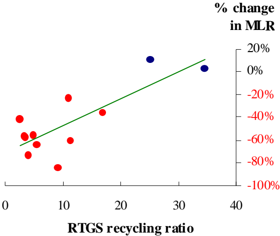
Figure 7.13 Impact of RTGS recycling ratio on banks' total liquidity requirements under RRGs Payments \geq £1bn time-critical
