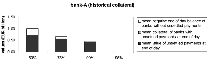
Figure 5.10 The average values of bank-A using historical collateral amounts for 50%, 75%, 90% and 95%, with each day treated individually.
