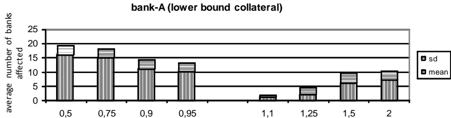
Figure 5.6 Average number of bank affected when bank-A pays 50%–95% and 110%–200% of its payments, with each day treated individually and the lower bound collateral amount being used by all banks
