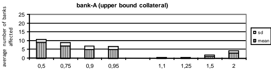
Figure 5.5 Average number of bank affected when bank-A pays 50%–95% and 110%–200% of its payments, with each day treated individually and the upper bound collateral amount being used by all banks
