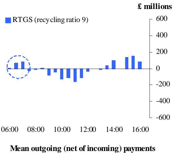
Profile of payments sent under RTGS (net of incoming payments) for Bank B: mean value at half an hour intervals across the month
