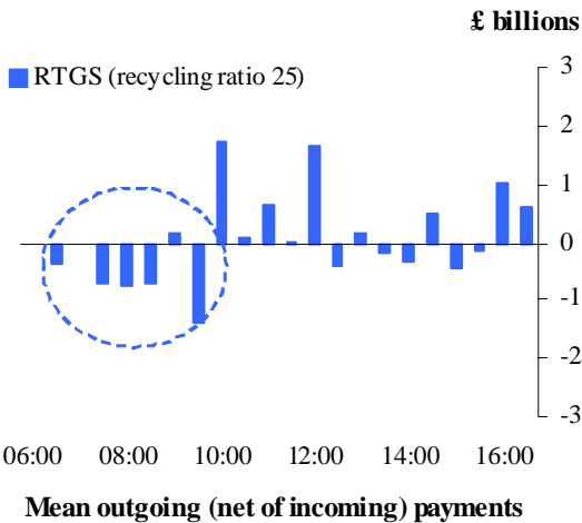
Profile of payments sent under RTGS (net of incoming payments) for Bank A: mean value at half an hour intervals across the month
