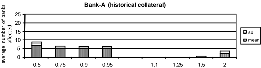
Figure 5.4 Average number of bank affected when bank-A pays 50%–95% and 110%–200% of its payments, with each day is treated individually and historical collateral amounts are used by all banks
