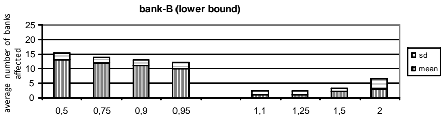
Figure 5.8 Average number of bank affected when bank-B pays 50%–95% and 110%–200% of its payments, with each day treated individually and the lower bound collateral amount used by all banks
