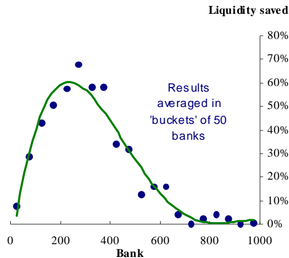
Figure 7.4 Mean liquidity savings under RRGs Bank sizes and payment values log-normally distributed – largest 5% of payments time-critical
