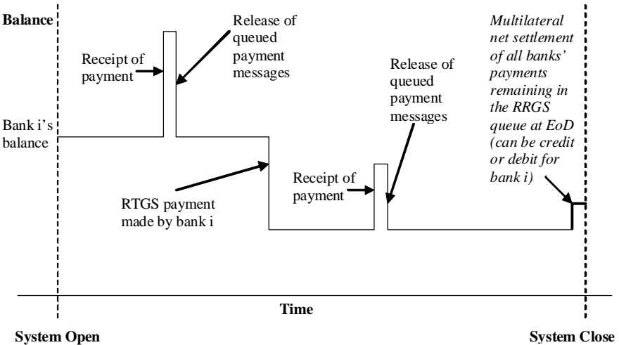
Figure 7.1 Dynamics of a bank’s balance under RRGs
