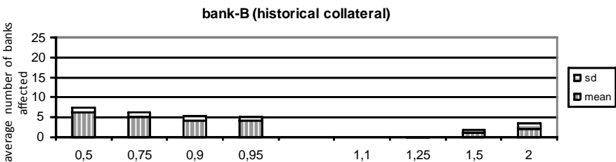
Figure 5.7 Average number of bank affected when bank-B pays 50%–95% and 110%–200% of its payments, with each day treated individually and historical collateral amounts are used by all banks
