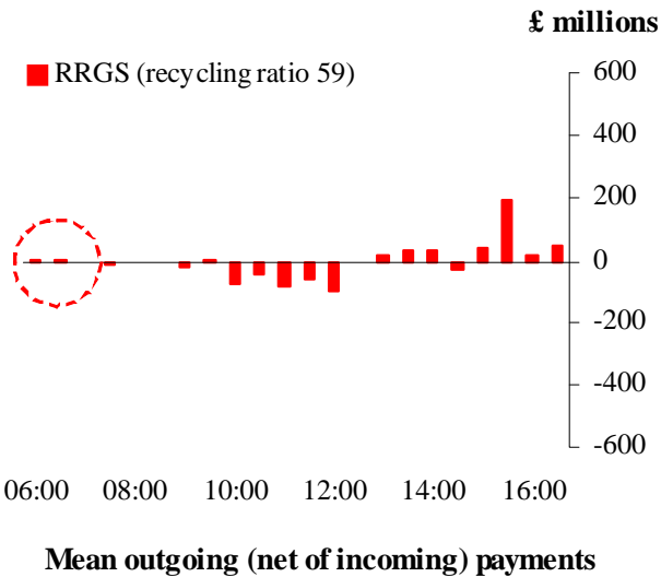
Profile of payments sent under RRGs (net of incoming payments) for Bank B: mean value at half an hour intervals across the month
