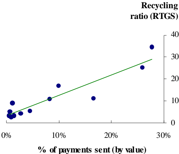
Relationship between banks' total payment value sent and recycling ratio under RTGS
