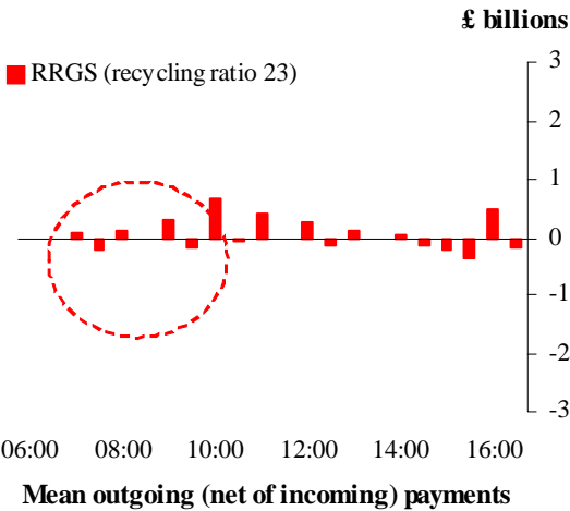
Profile of payments sent under RRGs (net of incoming payments) for Bank A: mean value at half an hour intervals across the month
