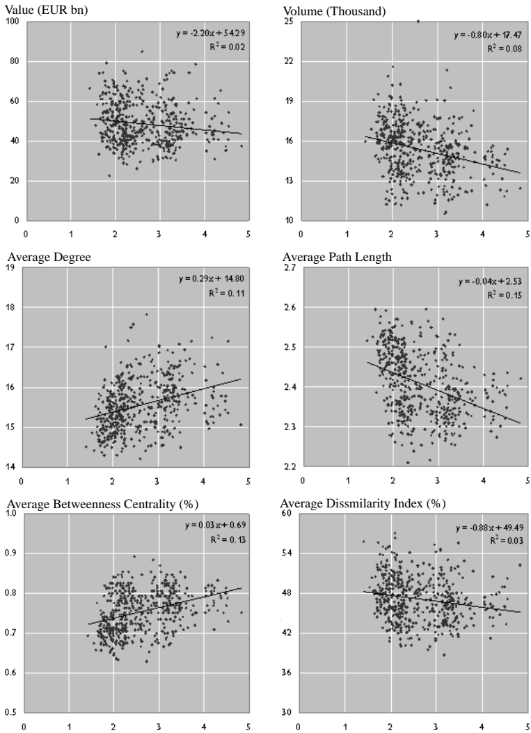
Figure 6.2 ARTIS Network Indicators (Network-level) vs Contagion (Daily Average of Number of Participants with Unsettled Payments across Scenarios)
