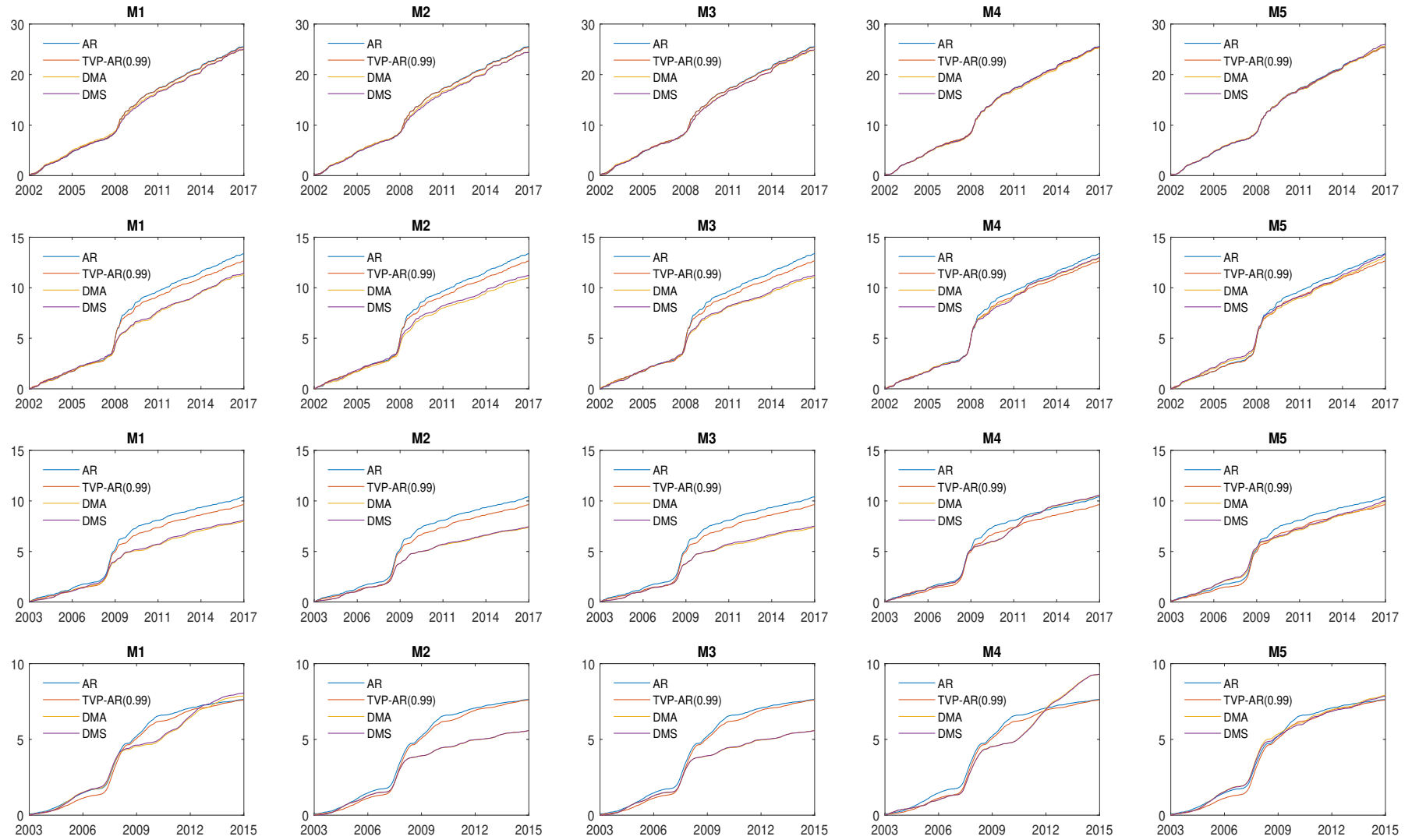
Figure 3: Cumulated absolute forecast error for each model. The four rows correspond to h \in \{1, 3, 6, 12\} .
