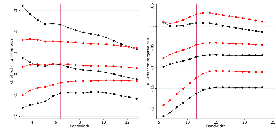
Figure 7: Controlling for predetermined covariates
