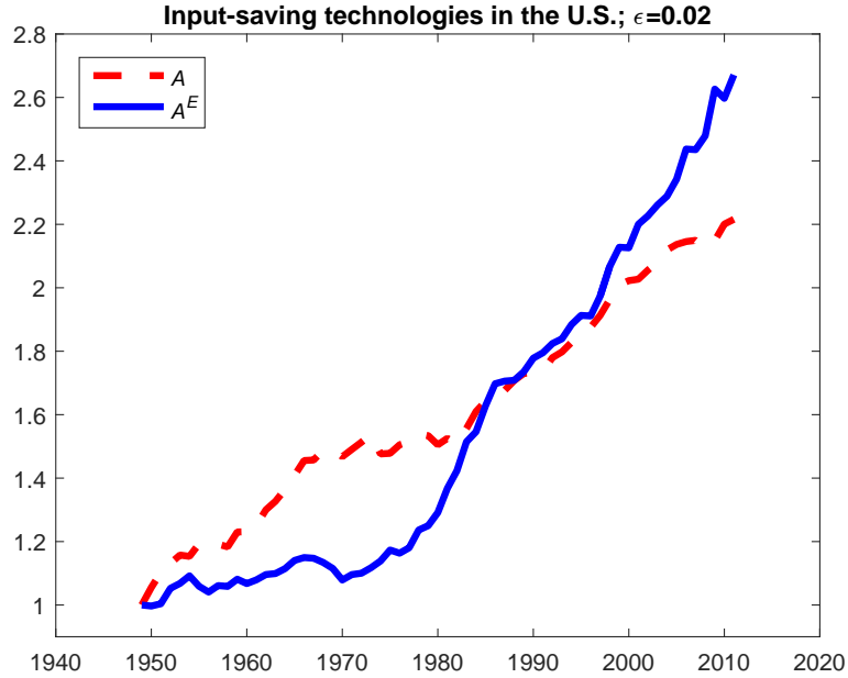
Figure 3: Energy- and capital/labor-saving technologies compared.
