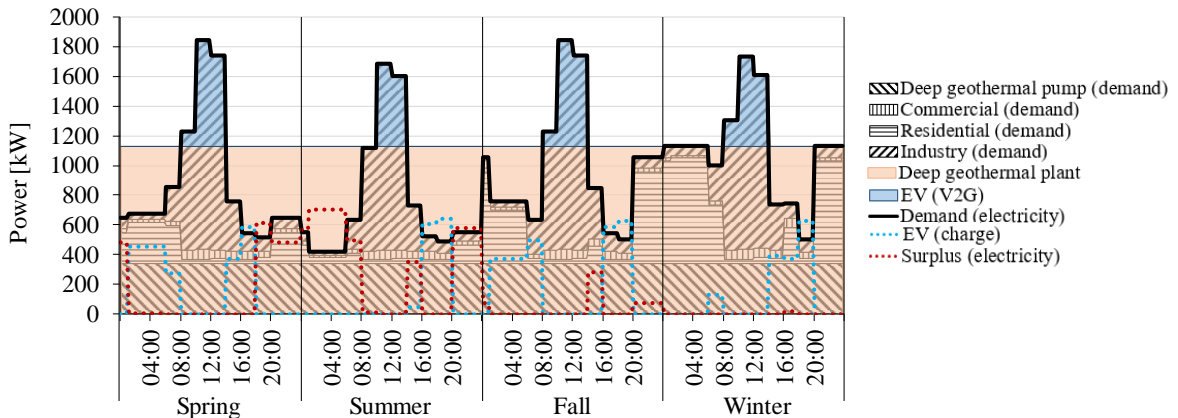
Fig. 2: Electricity generation and demand patterns for a typical weekday in all four seasons in 2015.
