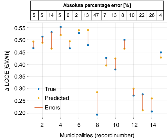
Fig. 3: Results of the stepwise linear regression. The error margins between the results from the optimizations (true) and the predicted values from the regression are shown.
