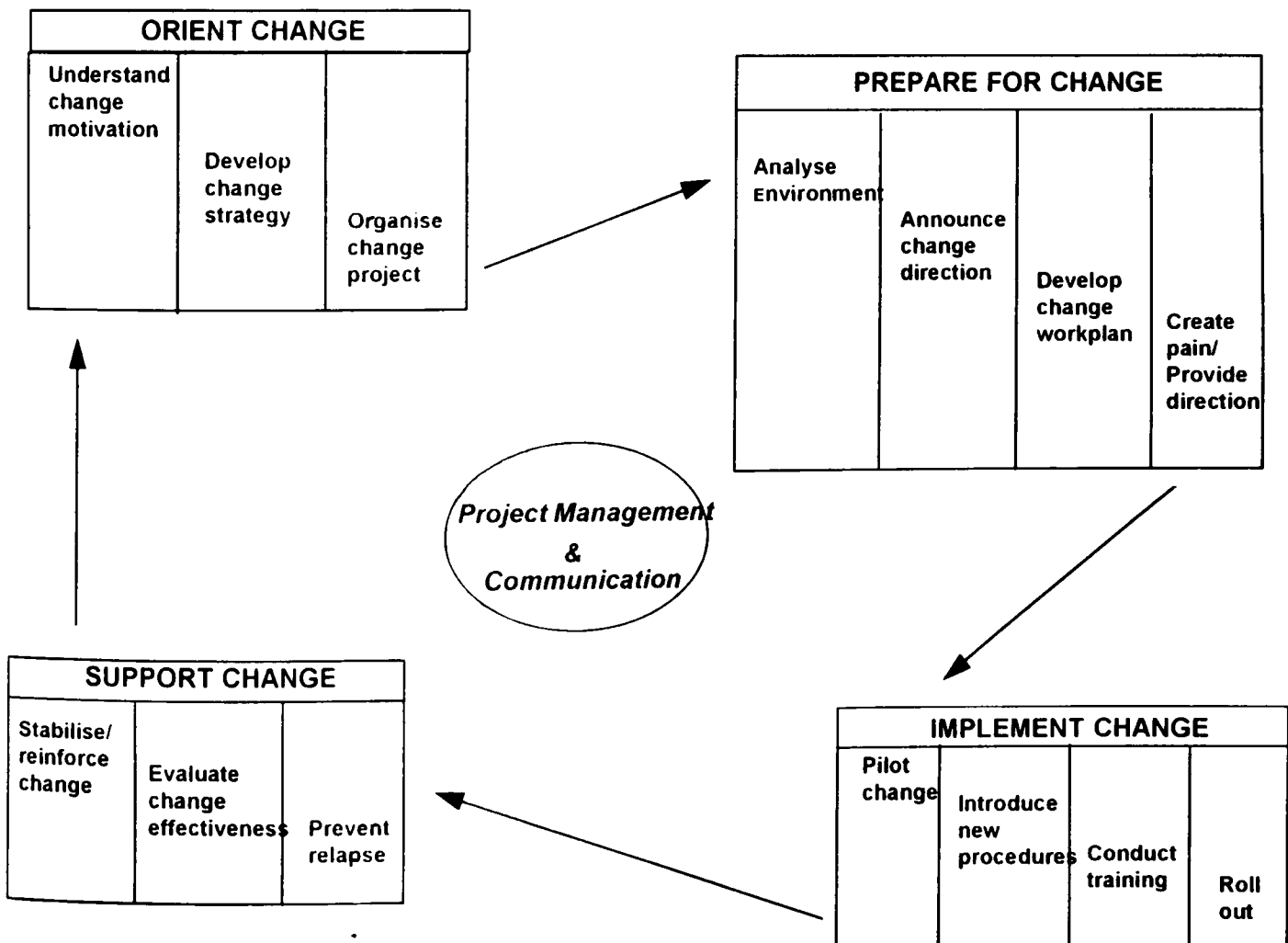
Figure 1 SDLC phases
