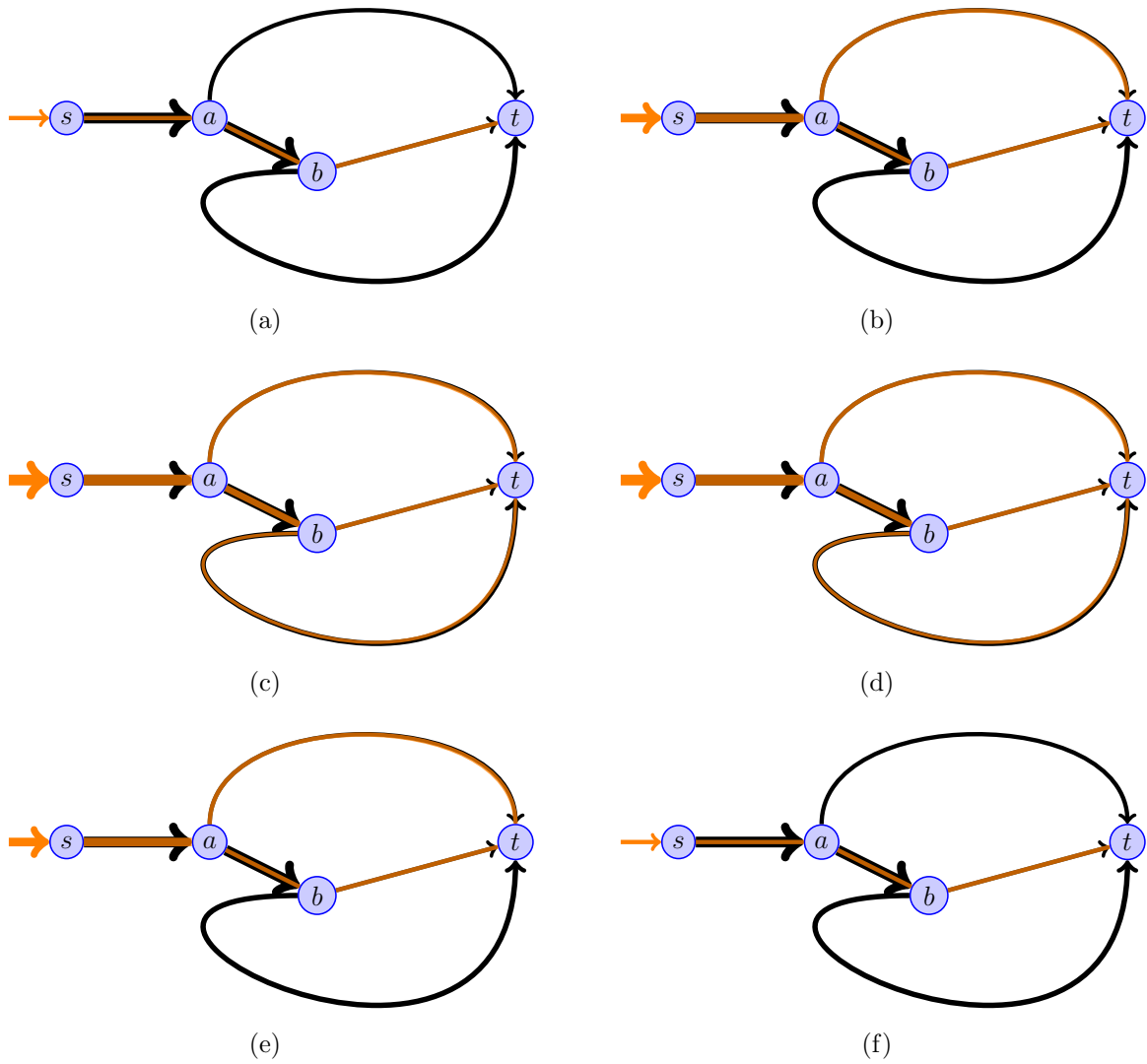
Figure 8: Chronological evolution with tolls: in orange the routes that the agents arriving at t have taken.
