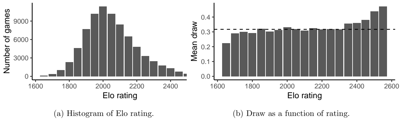
Figure A1: Frequency of Elo rating and draw per rating.
