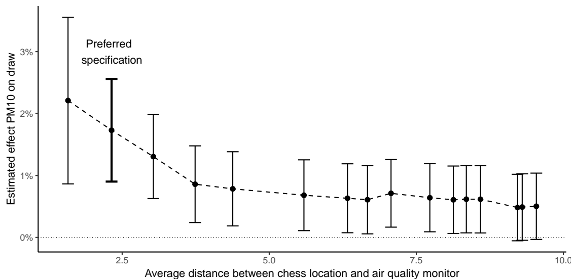
Figure 2: Sensitivity to distance between chess game and air quality monitoring station (error bars indicate 95% confidence intervals).
