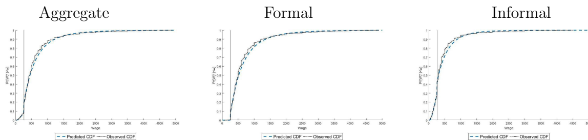
Figure 9: Observed and Predicted CDFs
