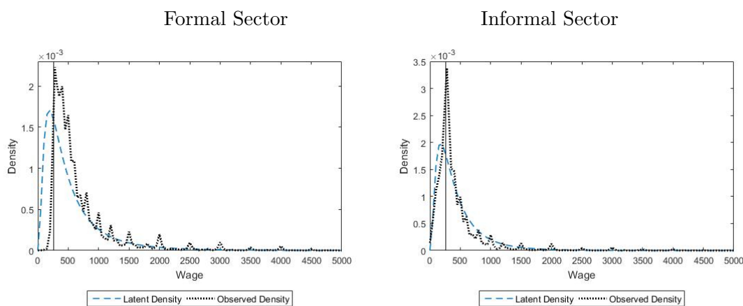
Figure 8: Latent and Observed Densities
