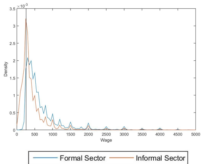
Figure 2: Observed Densities
