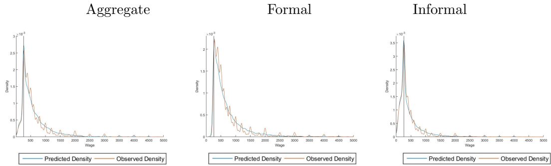
Figure 3: Model Fit
