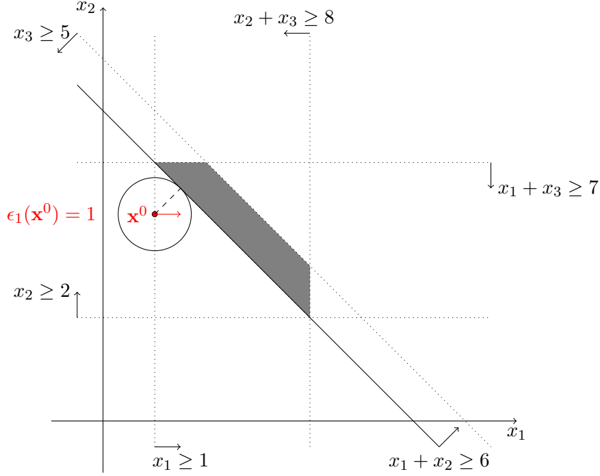
Figure 4: Hyperplane of preimputations: x_1 + x_2 + x_3 = v(\mathcal{N}) = 12
