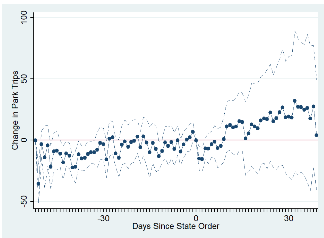
Figure 8: Parks
