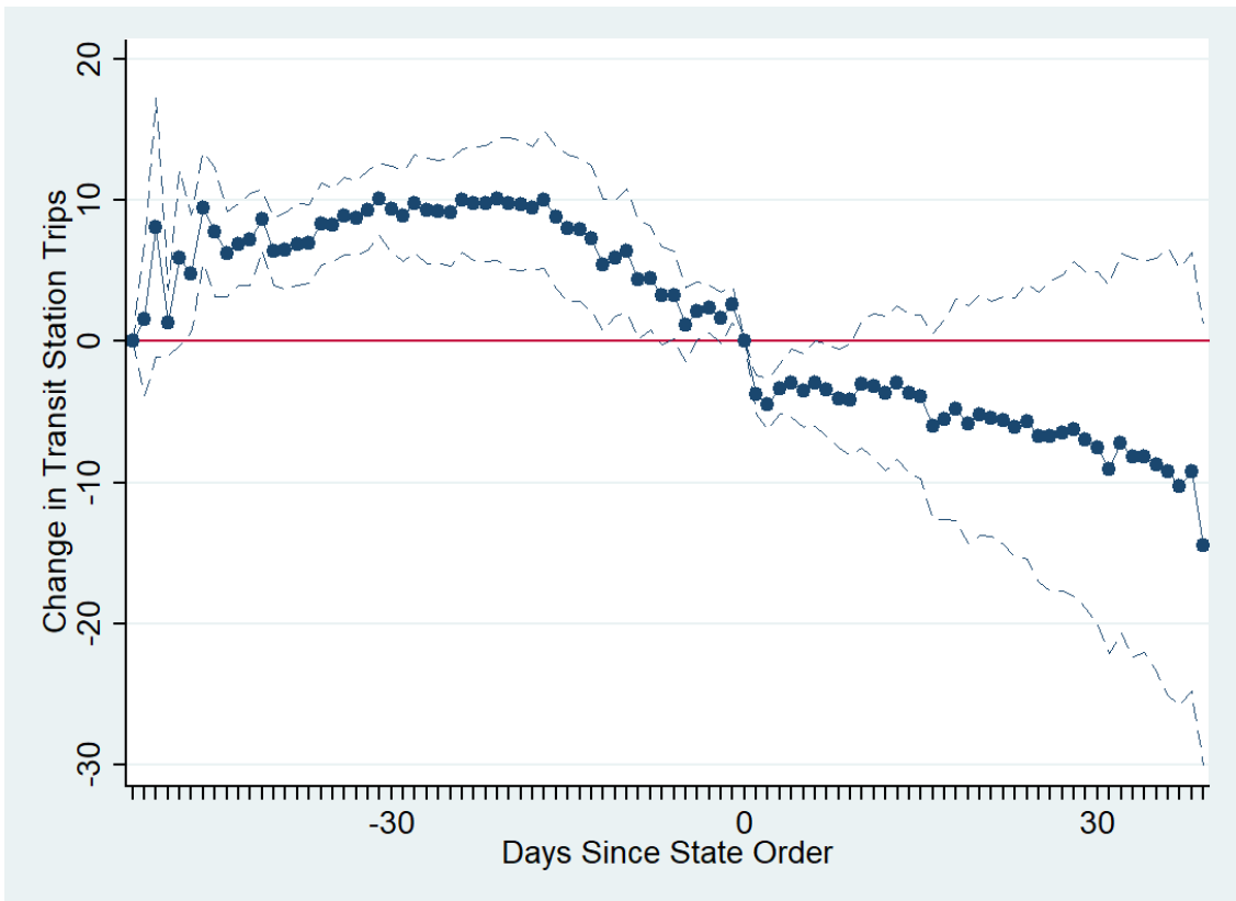
Figure 9: Transit Stations
