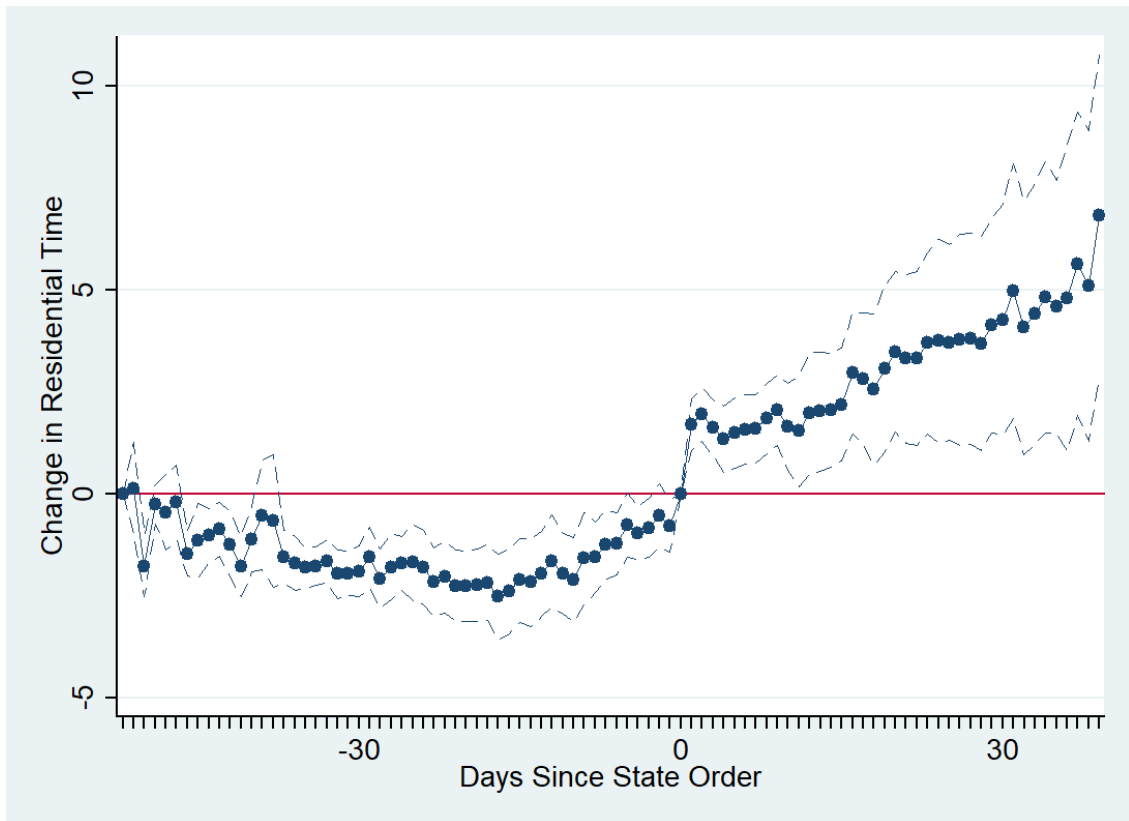
Figure 11: Residence
