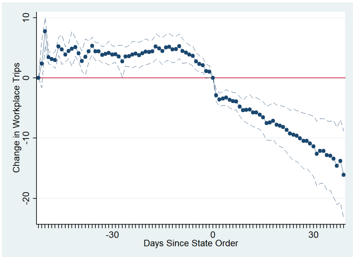
Figure 10: Workplaces
