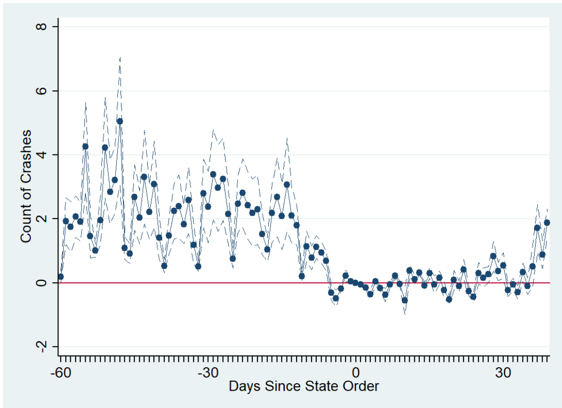
Figure 12: Traffic Collisions
