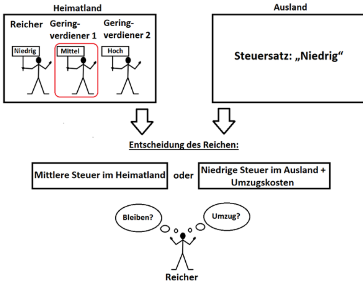
Figure 4: Instruction example
