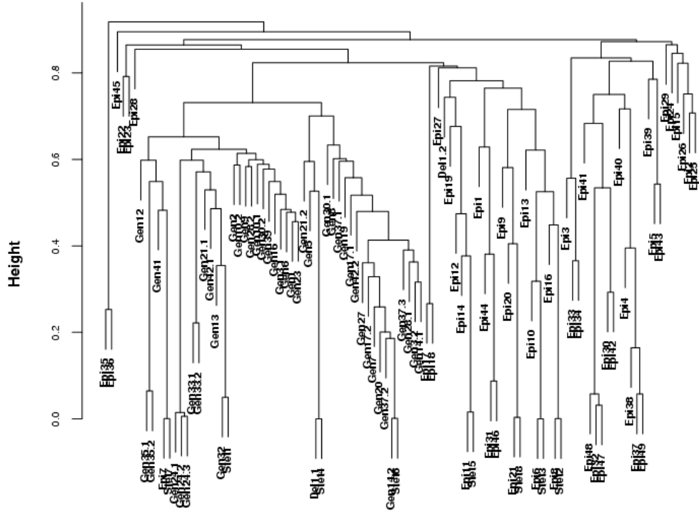
Figure 10. Dendrogram of S^{block} of the SNP loci and the epidemiological variables of the control group according to ii and using S_e .
