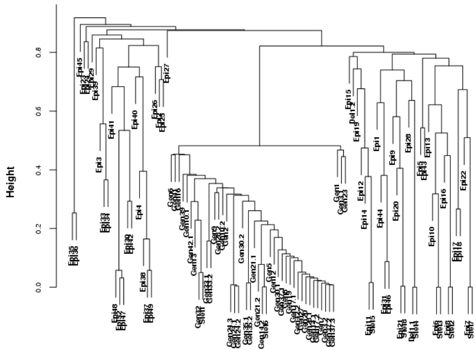
Figure 11. Dendrogram of S^{block} of the SNP loci and the epidemiological variables of the control group according to iii and using S_e .
