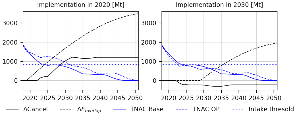
Figure 3: Cumulative overlapping emission reductions ( \Delta E_{overlap} ), change in TNAC volumes and cumulative change in cancellation ( \Delta Cancel ) for implementing overlapping policies in 2020, left, and 2030, right.
