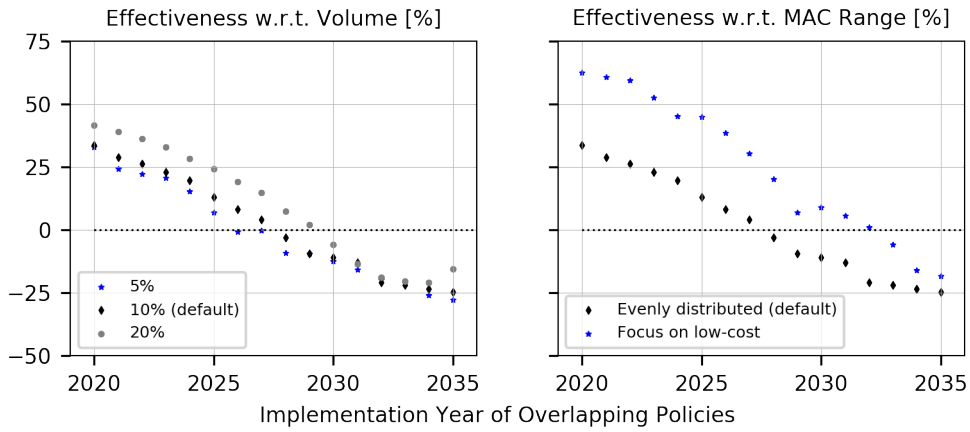
Figure 5: Effectiveness for different addressed volumes of overlapping policies (as share of baseline emissions), left, and different designs, right.
