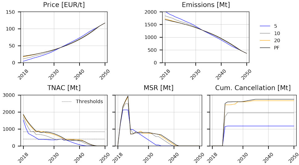
Figure D.7: Market outcomes for the base scenario under myopia (for planning horizons of 5,10 and 20 years) compared to the results under Perfect Foresight (PF).
