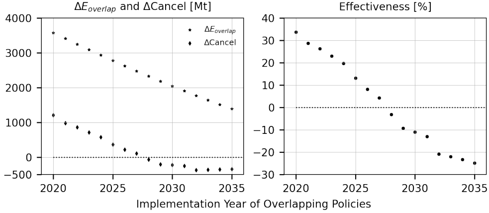
Figure 4: Overlapping emission reduction ( \Delta E_{overlap} ), additional cancellation ( \Delta Cancel ), both left, and effectiveness, right, for different implementation years of overlapping policies.
