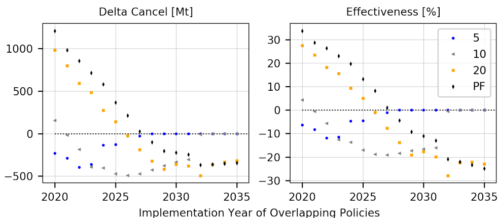
Figure 6: Additional Cancellation and Effectiveness of depending on timing and planning horizon.
