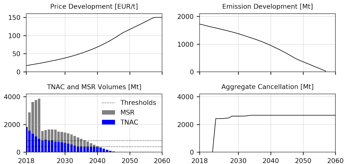
Figure 2: Prices, emissions, banking and total cancellation in the base scenario.
