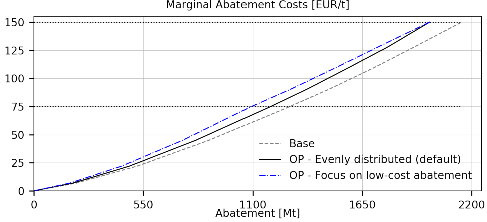
Figure 1: Marginal abatement cost curves without ( base ) and with overlapping policies ( OP - Evenly Distributed and OP - Focus on Cheap Abatement ).
