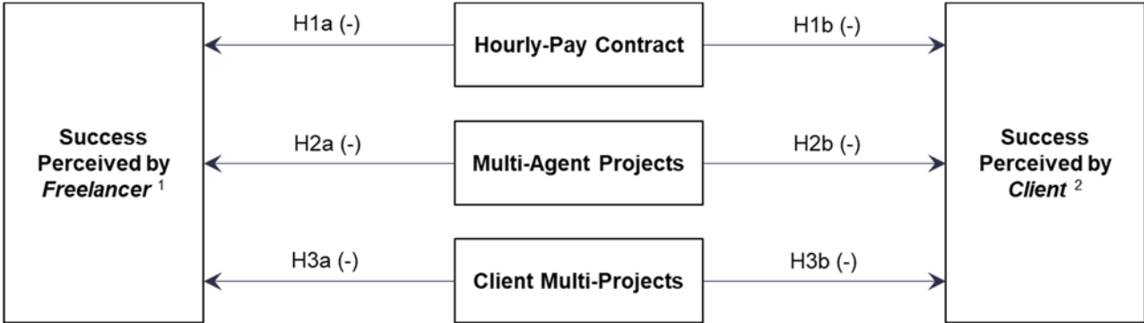
Figure 1: Empirical Model
