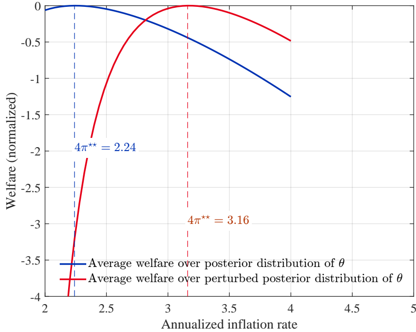
Figure 12: \mathbb{E}_\theta(\mathcal{W}(\pi, \theta))
