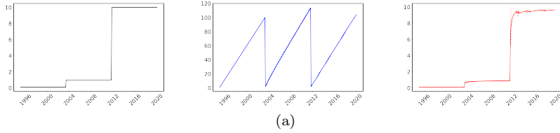
Figure 4: Simulated series (left), homogeneous windows (middle) and MLE (right) using arithmetically increasing intervals in LPA. LPA_Simulations
