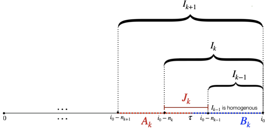
Figure 2: Iterative algorithm
