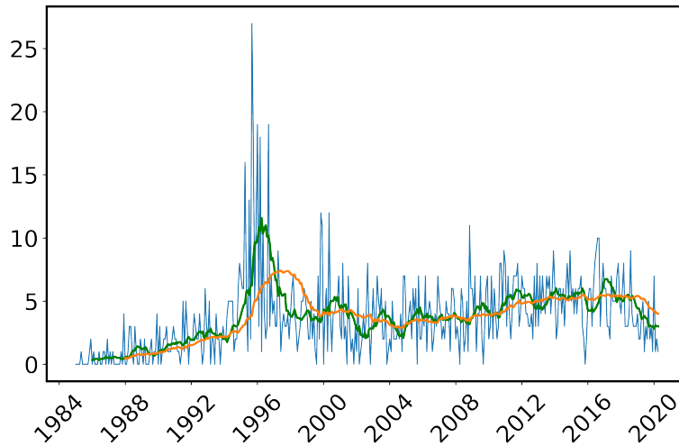
Figure 1: Time series of count of mergers and acquisitions per month, with moving average curve of 1 year and 3 years. LPA_Empiricalstudy
