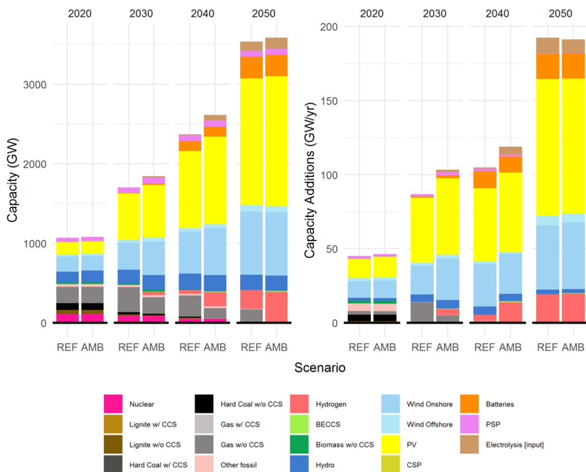
Figure 2: Capacities (left) and capacity additions (right) in REF and AMB (assuming default demand and default transmission expansion) between 2020 and 2050 in the EU ETS.
