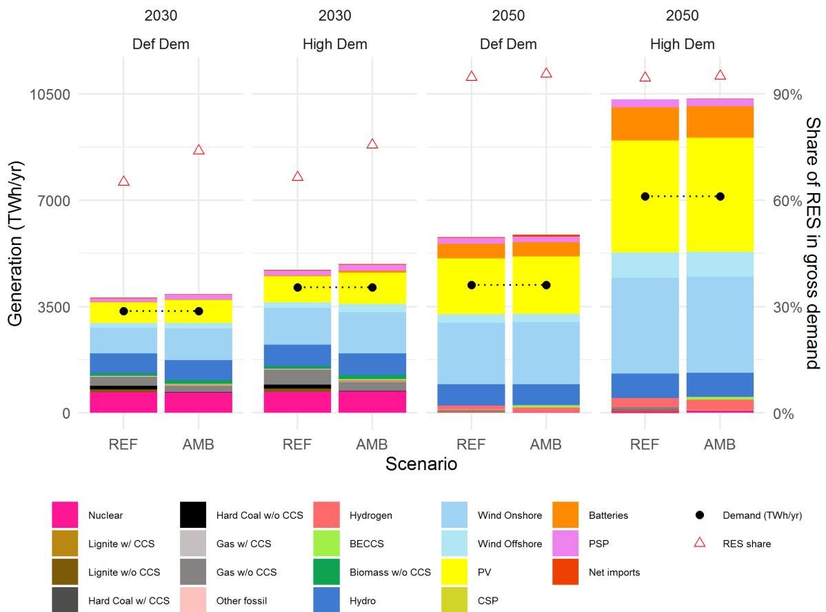
Figure 6. Generation-mix in the EU ETS in 2030 and 2050 for the scenarios with default and high demand (assuming unrestricted transmission expansion) in the EU ETS.
