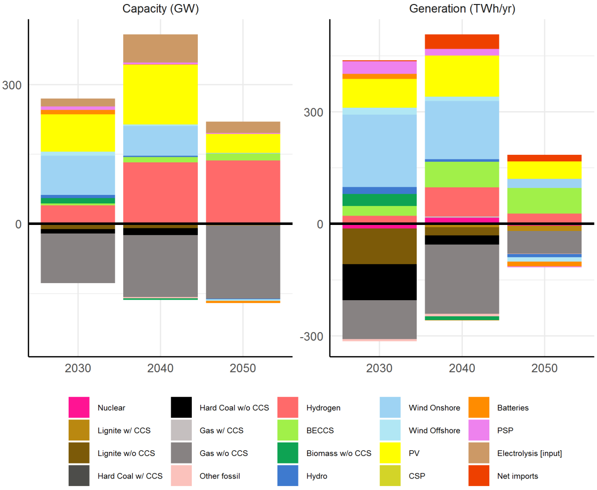
Figure 3. Difference in capacity- and generation-mix between AMB and REF in the EU ETS. Positive values mean higher capacity/generation in AMB.
