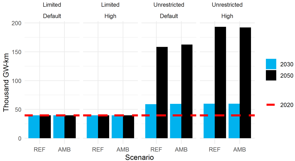
Figure 7. Aggregate transmission capacity at the EU ETS level in 2030 and 2050.
