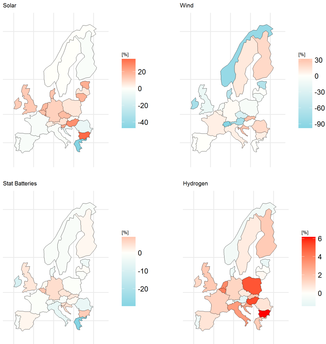
Figure 10. Impact of transmission grid expansion on the generation-mix. The colour legend indicates the change in the 2050 share of this technology's output in gross demand when going from AMB with default transmission expansion to AMB with no transmission expansion. A positive value implies that the share of the technology is higher in the scenario with limited transmission expansion than in the one with unrestricted transmission expansion.
