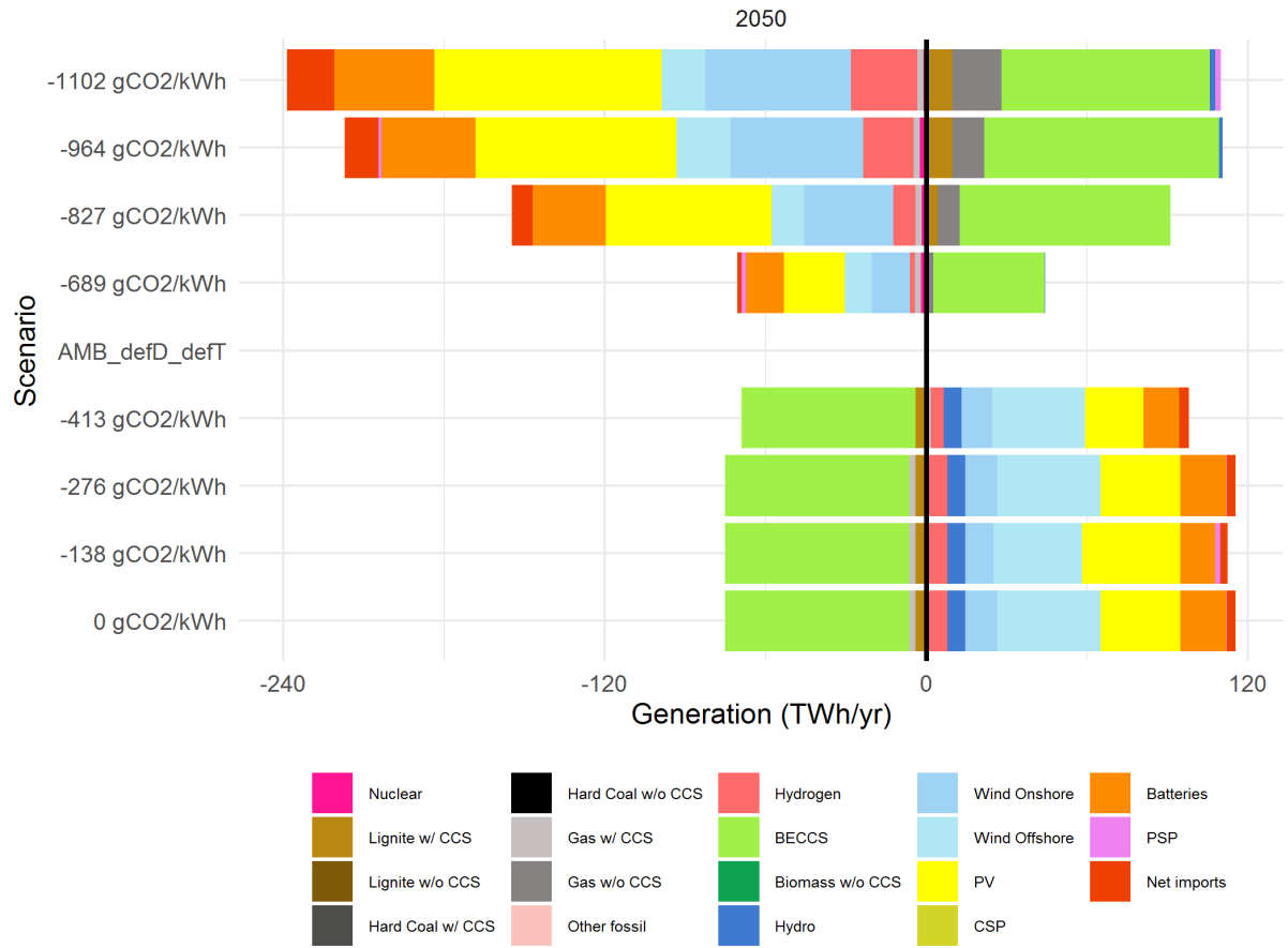
Figure 13. Change in generation in 2050 between BECCS emission factor scenarios and default AMB scenario (-551 gCO 2 /kWh el ) in the EU ETS. A positive value means there is higher generation in the corresponding scenario.
