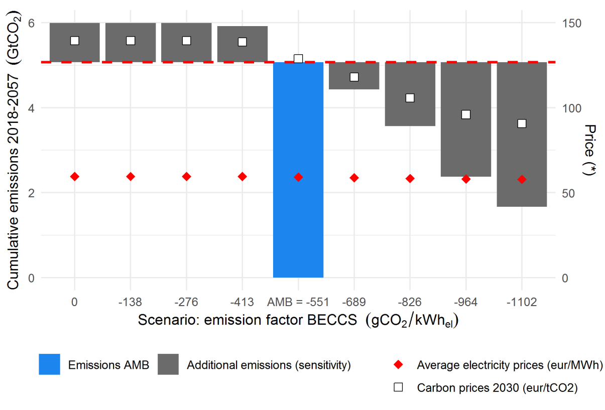
Figure 12. Impact of the BECCS emission factor on power sector emissions (left axis), carbon prices in 2030 and average electricity prices (right axis) in the ambitious scenario (assuming a default demand and unrestricted transmission expansion) in the EU ETS.
