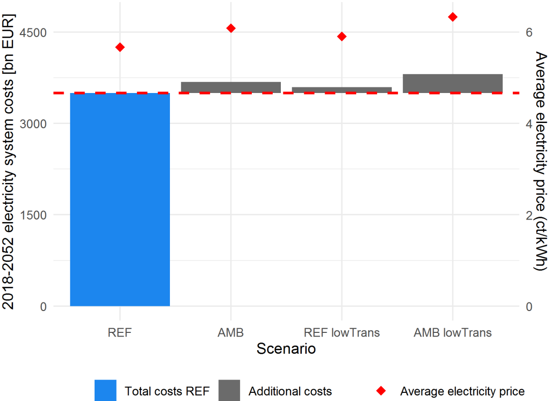
Figure 8. Total discounted cost of the electricity sector 2018-2052 and average electricity price in REF and AMB (assuming default demand), with the impact of low transmission in the EU ETS.
