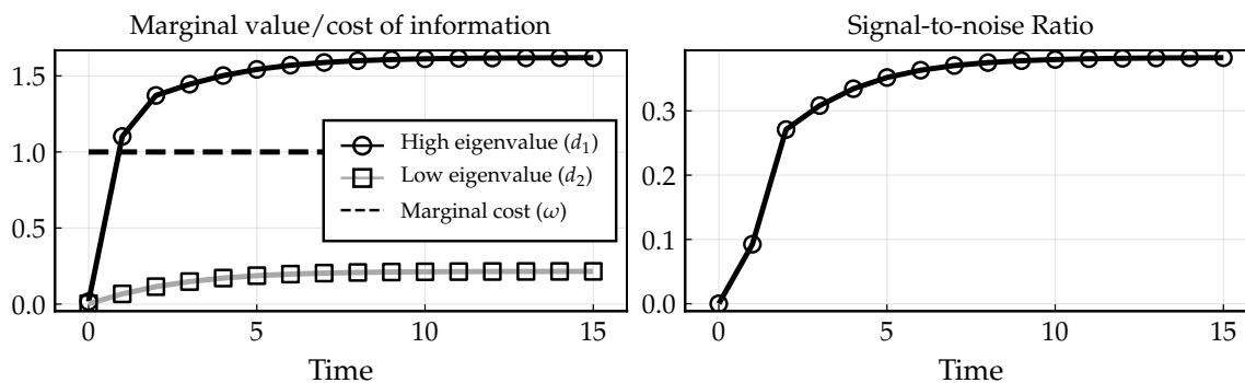
Figure 1: Transition Dynamics of Attention
