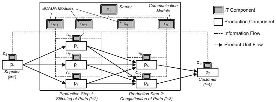
Fig. 4 Exemplary smart factory
