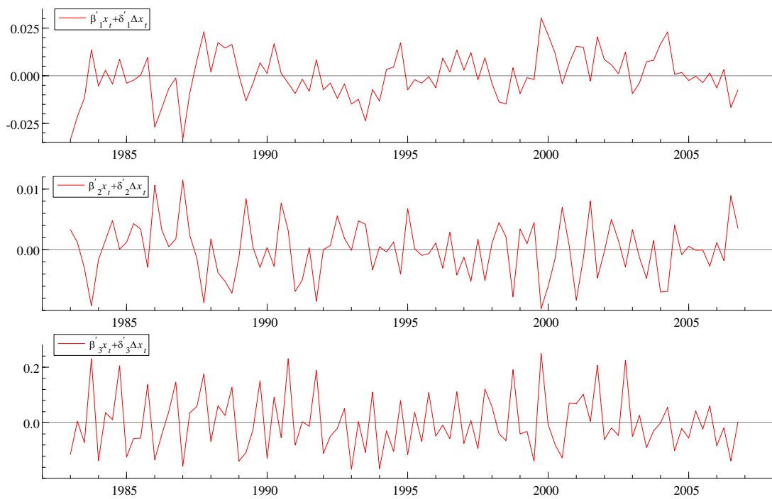
Figure A.2: Model II: Multi-cointegrating relations (means-corrected).
