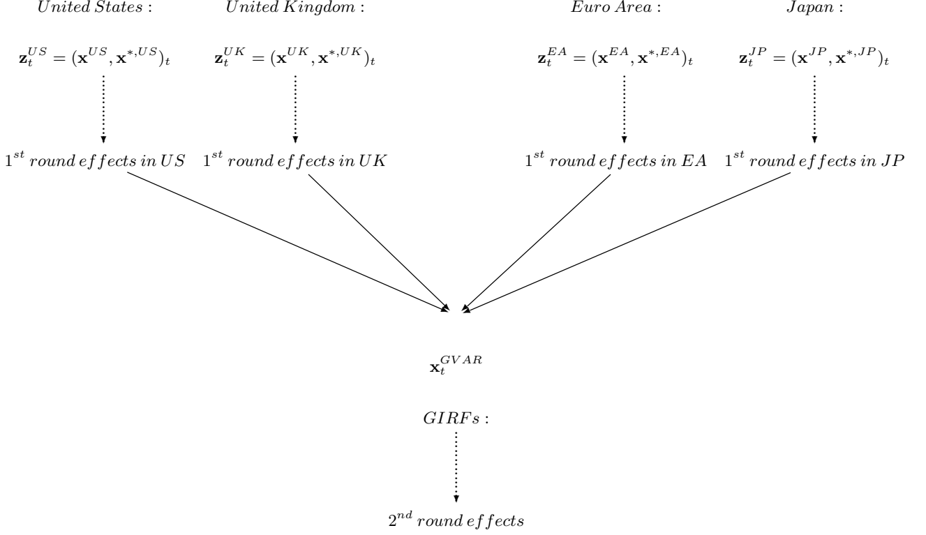
Figure 1: Global VAR procedure for shocks analysis.
