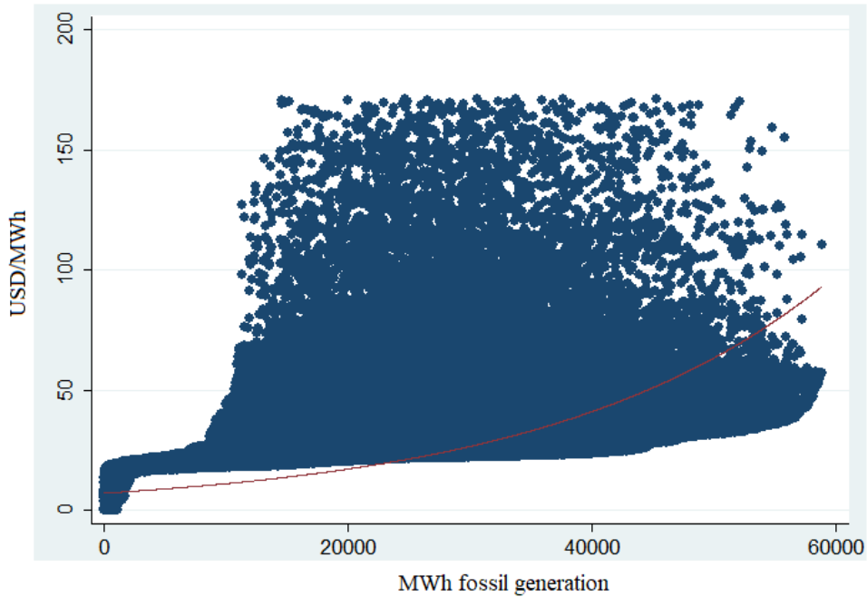
Figure 2. Private Fossil Generation Marginal Costs in ERCOT
