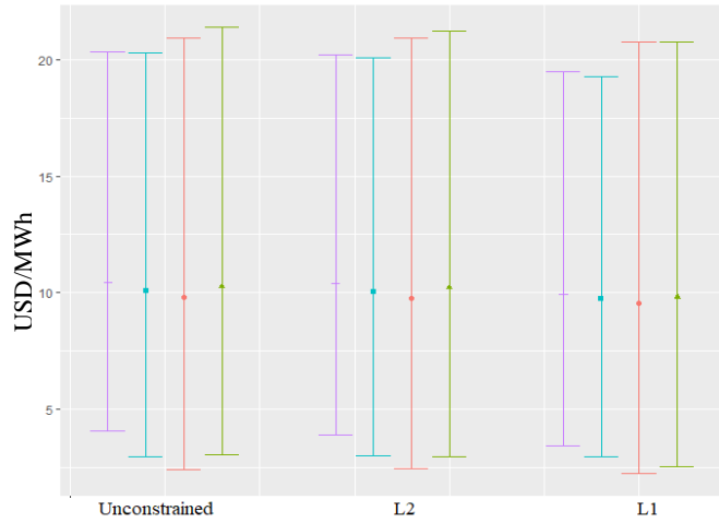
5c. Air pollution marginal damages of EV charging scenarios
