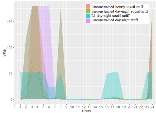
4c. Day-night tariff charging
