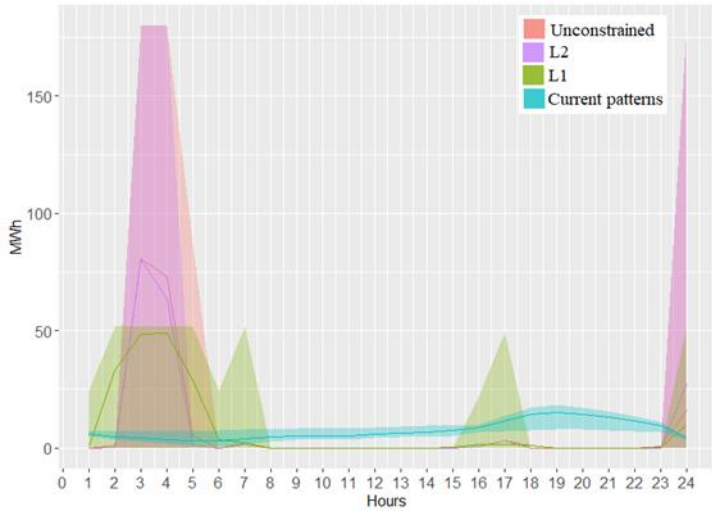
4a. Welfare-maximizing charging (hourly tariff)
