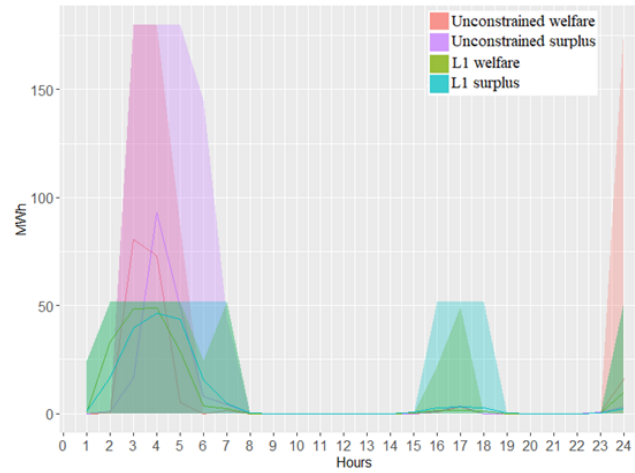
4c. Day-night tariff charging
