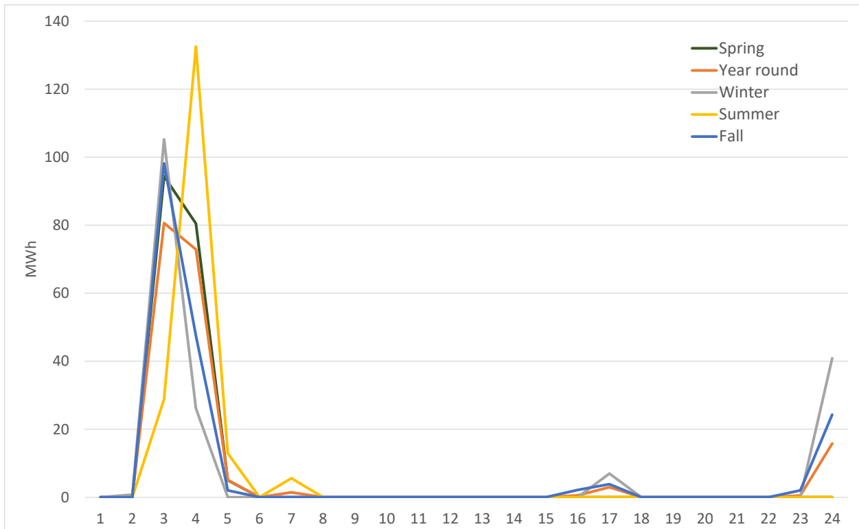
Figure 6. Average Seasonal EV Charging Schedules (unconstrained welfare maximizing)
