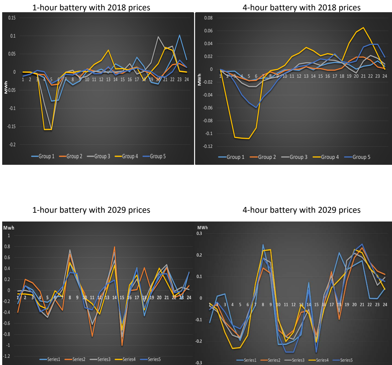
Figure 6. Clusters of Daily Optimal Charging and Discharging Actions
