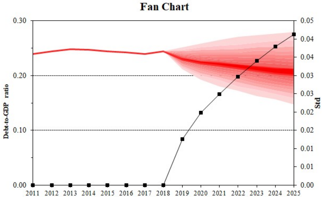
Figure 16. VAR-Model Projections
