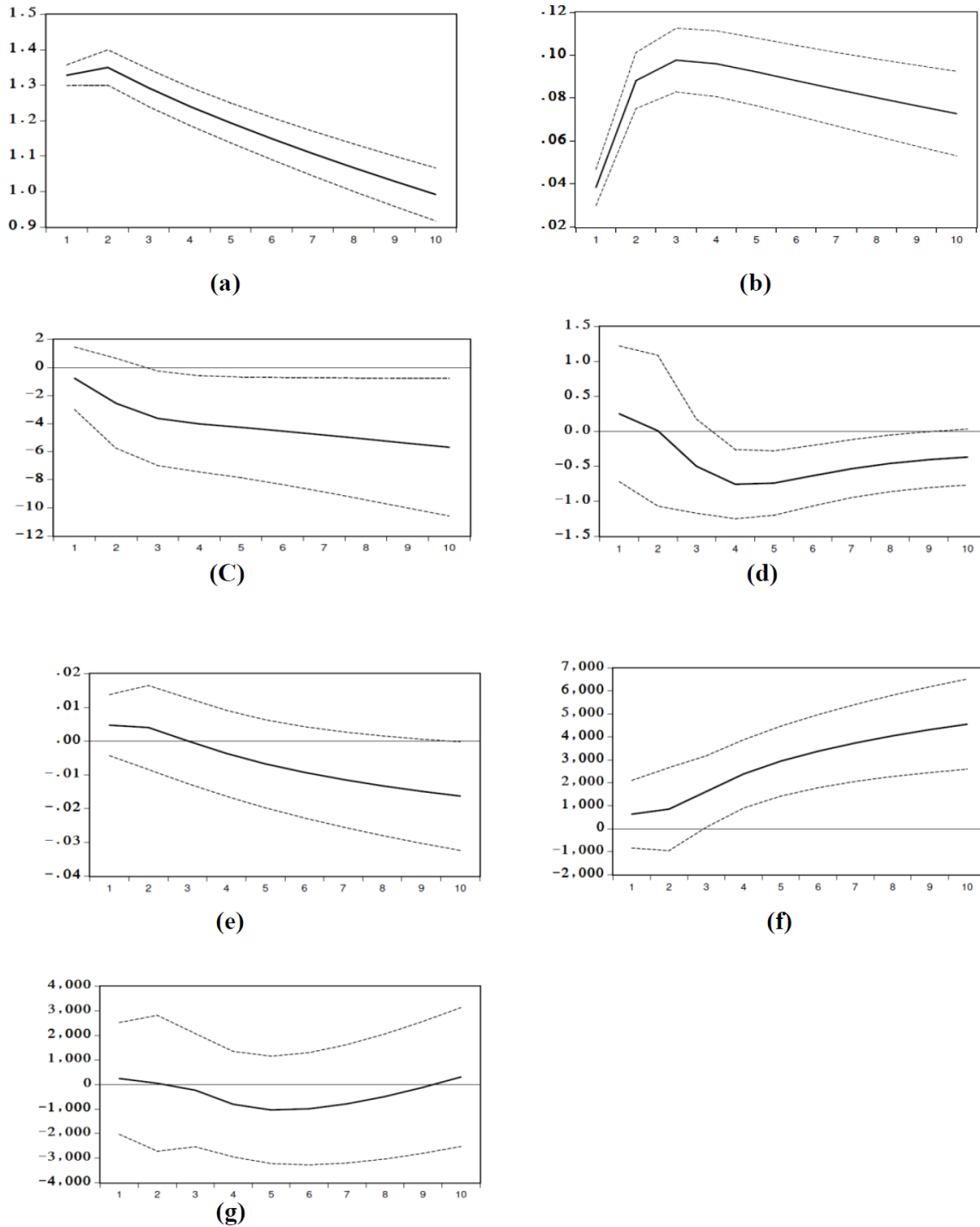
Fig.3 Impulse response functions related to a one-standard-deviation positive shock in Polity2 index. a Response of Polity2 index. b Response of military in politics index. c Response of military expenditures (per capita). d Response of arms imports (per capita). e Response of armed forces personnel (% of total labor force). f Response of non-defense expenditure (per capita). g Response of government revenue (per capita). Notes: The dotted lines represent \pm 1 standard deviation. The horizontal axis shows the time periods (years) after the initial shock. The magnitude of the responses is presented on the vertical axis.
