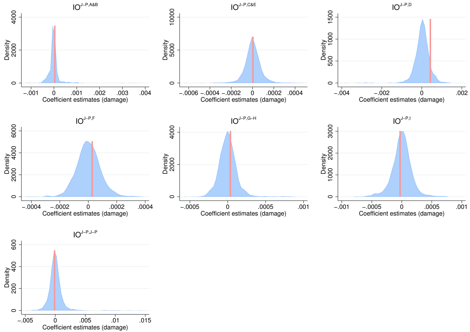
Figure 25: Randomization tests for Input-Output coefficients of sector aggregate J-P. This figure shows the Fisher randomization test results for the damage t variable where the years are permuted for 2000 repetitions. It displays the kernel density plots (blue) of the randomization coefficient estimates together the results of model 6 (red bar). The sector abbreviations represent the following sector aggregates: agriculture, hunting, forestry, and fishing (A&B), mining, and utilities (C&E), manufacturing (D), construction (F), wholesale, retail trade, restaurants, and hotels (G-H), transport, storage, and communication (I), other activities (J-P).
