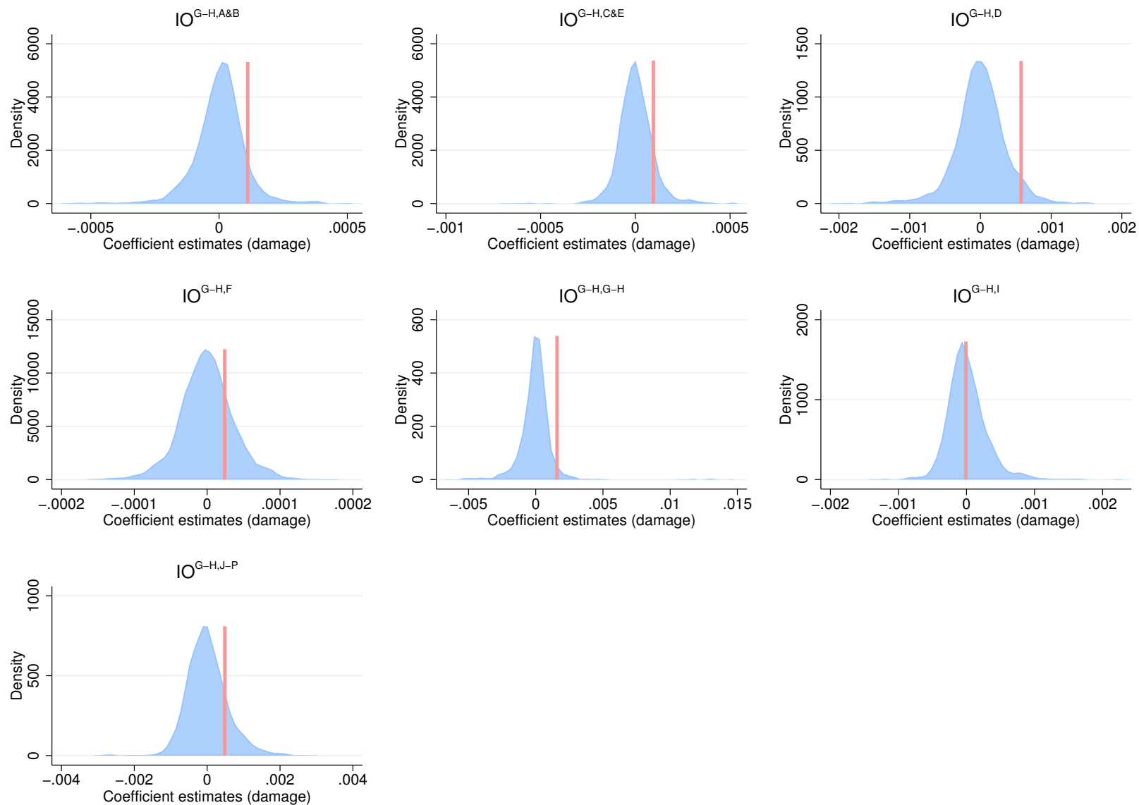
Figure 23: Randomization tests for Input-Output coefficients of sector aggregate G-H. This figure shows the Fisher randomization test results for the damage t variable where the years are permuted for 2000 repetitions. It displays the kernel density plots (blue) of the randomization coefficient estimates together the results of model 6 (red bar). The sector abbreviations represent the following sector aggregates: agriculture, hunting, forestry, and fishing (A&B), mining, and utilities (C&E), manufacturing (D), construction (F), wholesale, retail trade, restaurants, and hotels (G-H), transport, storage, and communication (I), other activities (J-P).
