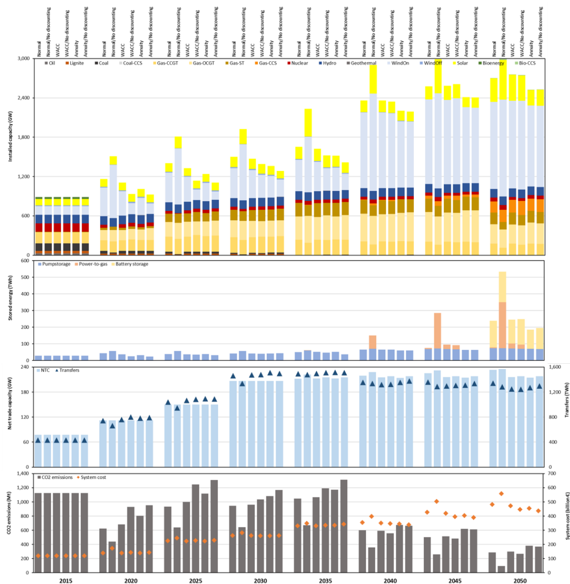
Evolution of installed capacity, storage, NTC and CO2 emissions and system cost for model with 12 regions are shown for respective period and configuration of investment cost
