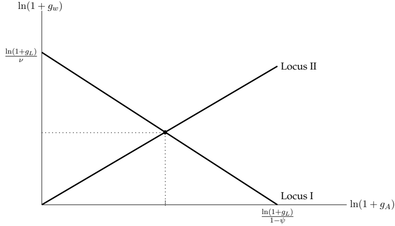
Figure 8.1: Steady-State Equilibrium.
