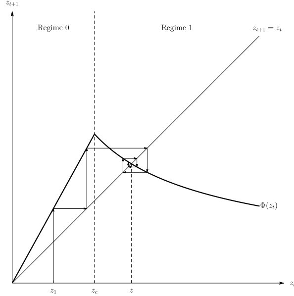
Figure 4.2: Case 2(a): Local and Global Dynamics of a Stable Steady-State Equilibrium for -\nu(\sigma - 1) \in (-(1 + \psi), -\psi) .
