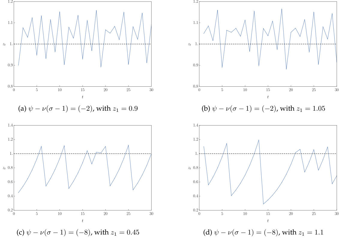
Figure 4.4: Four Possible Trajectories if -\nu(\sigma - 1) < -(1 + \psi) . Throughout, we set 1 + g_L = 1.006^{30} and choose parameters such that z_c = 1 .
