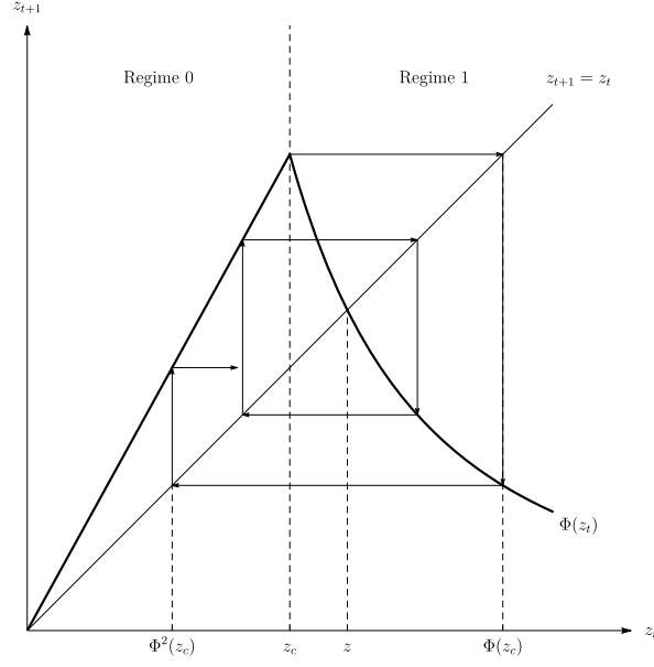
Figure 4.3: The Absorbing Interval and a 2 - Cycle Arising if -\nu(\sigma - 1) < -(1 + \psi) .
