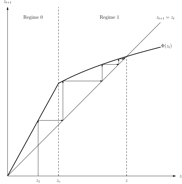
Figure 4.1: Case 1: Local and Global Dynamics of a Stable Steady-State Equilibrium for -\nu(\sigma - 1) \in (-\psi, 0) .
