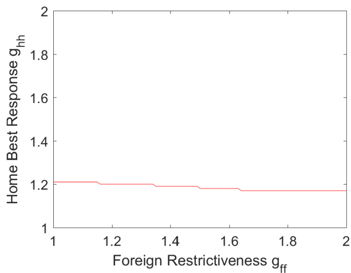
Figure 12: Best Response
