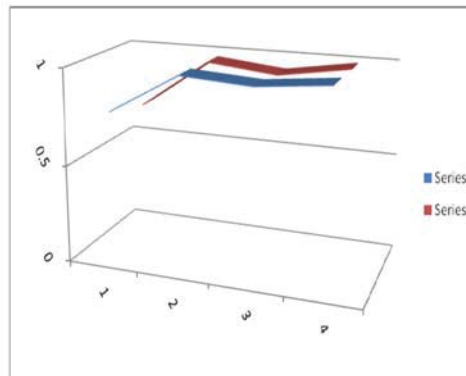
Figure-3. R^2 and R_{Adj}^2 for data set-2 for various models
