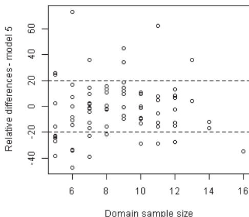
Figure 5 - Relative differences (%) by domain sample sizes - Model 5
