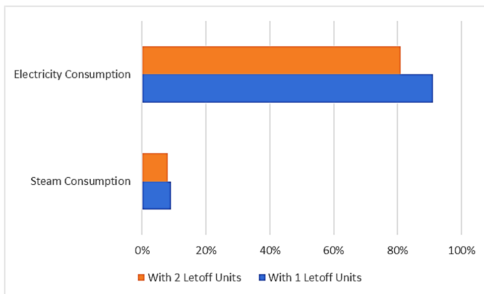
Figure 7. Electricity and steam savings (Source: Own study)
