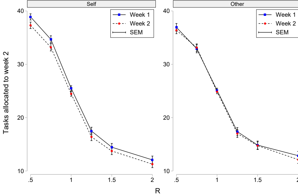
Figure 3: Effort allocations in intrapersonal decisions (SELF: n = 215 , OTHER: n = 214 )
