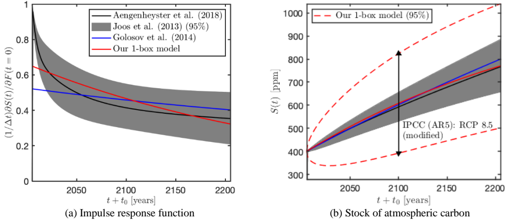
FIGURE 1. ATMOSPHERIC CARBON CYCLE AND UNCERTAINTY
