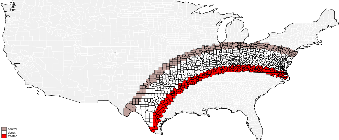
Figure A.6: Regression discontinuity design - map of treated and control counties
