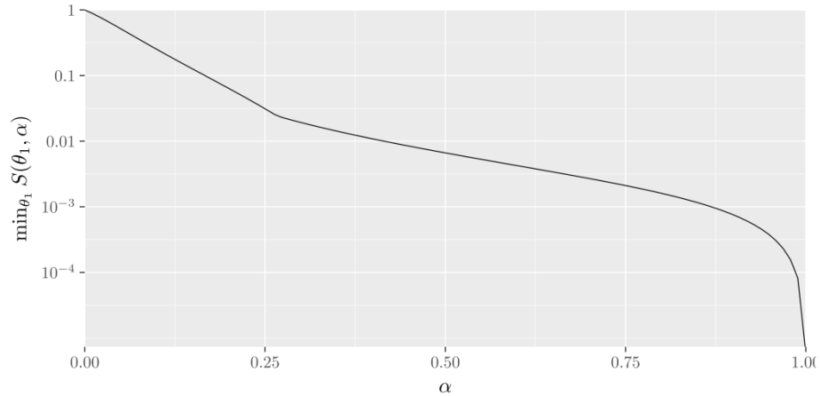
Figure 8.11 Stringency of the Most Stringent NP \alpha -level Test.
