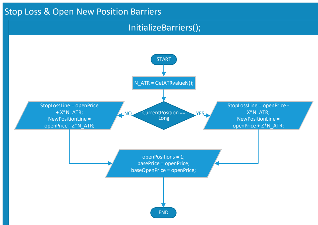
Figure 4. Initialization process after opening the first position. N_ATR is the ATR value at the time the position is opened, X is a constant adjusting the width of the stop loss zone and Z is a constant adjusting the width of the new position zone at which the trading strategy adds to the initial position.
